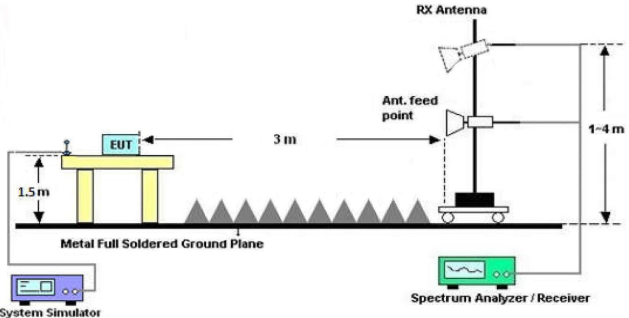
Figure 3. Above 1 GHz
