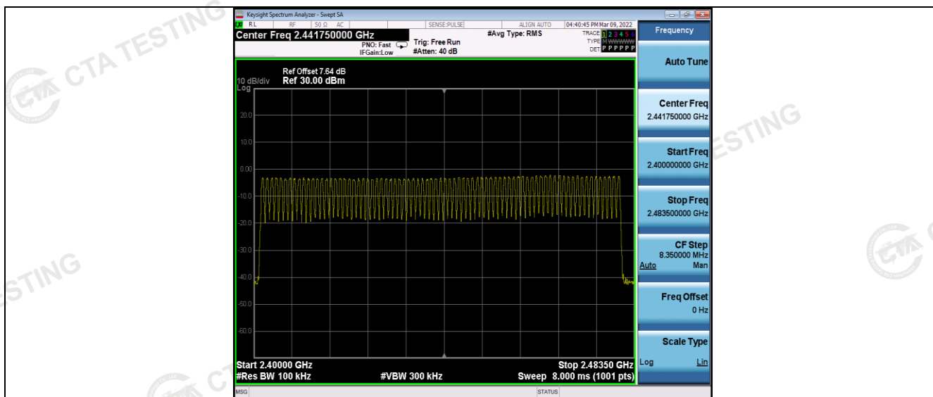
GFSK Modulation
