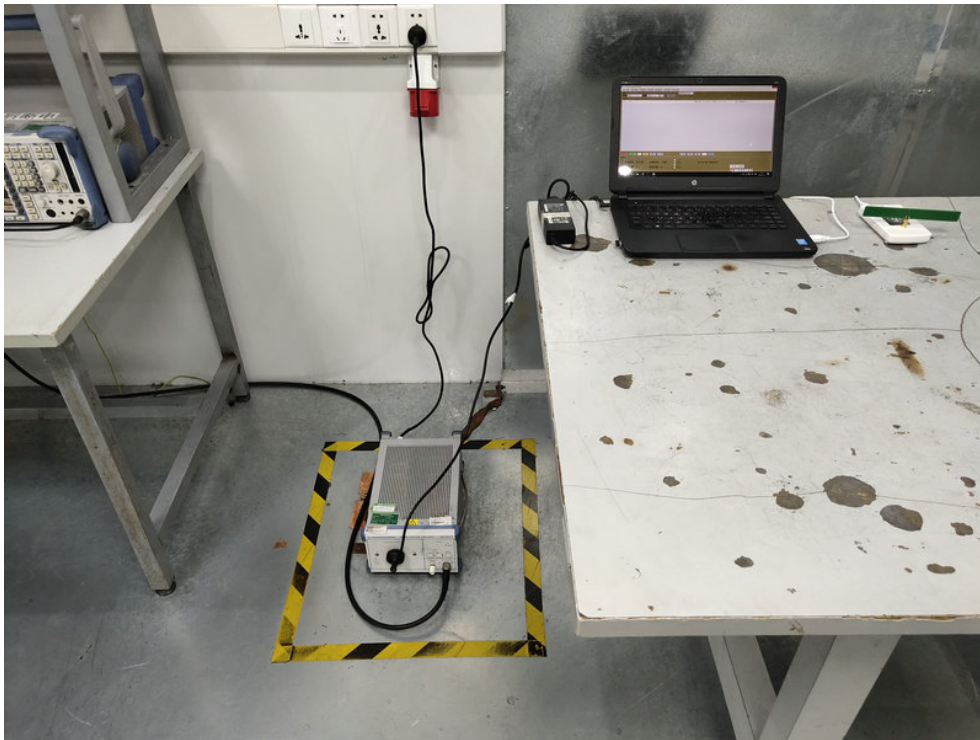
FCC ID: 2AV3T-FC01 Photo of Conducted Emission Measurement
