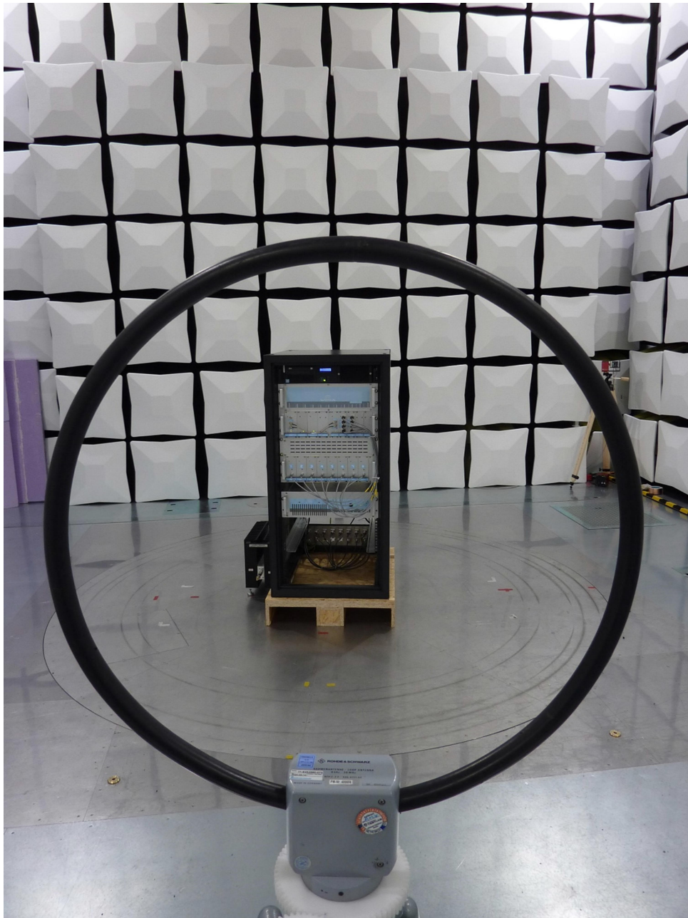
Test setup semi anechoic chamber 9 kHz – 30 MHz
