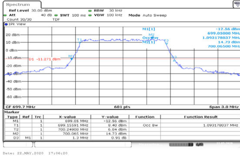
Band12-1.4MHz-QPSK-23095-6RB#0-1.093
