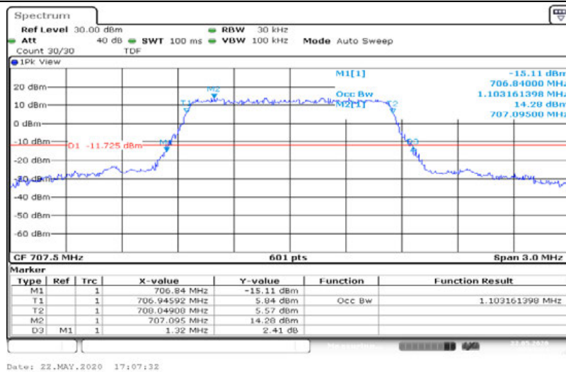
Band12-1.4MHz-16QAM-23173-6RB#0-1.103
