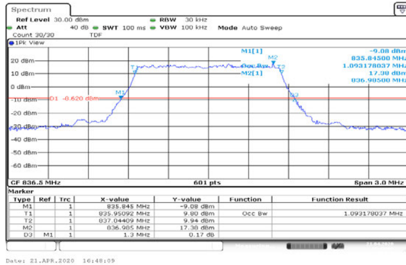
Band5-1.4MHz-QPSK-20643-6RB#0-1.093
