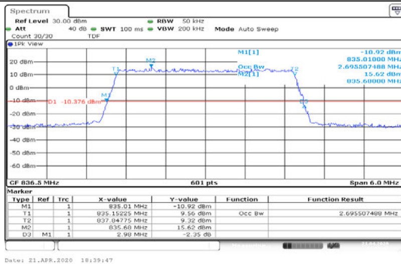
Band5-3MHz-16QAM-20635-15RB#0-2.696
