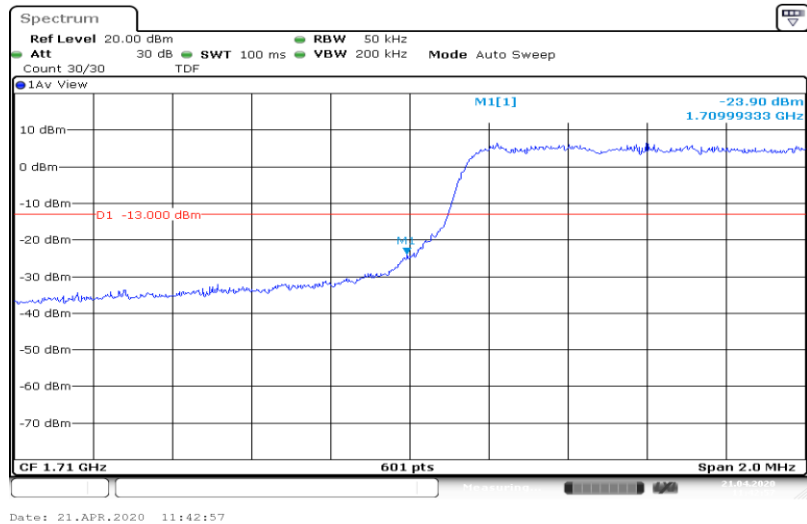
Band4-3MHz-16QAM-20385-15RB#0
