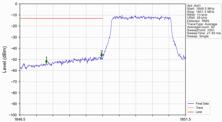
Band2_1.4MHz_16QAM_LCH_1850.7MHz_RB_6_0_NTNV
