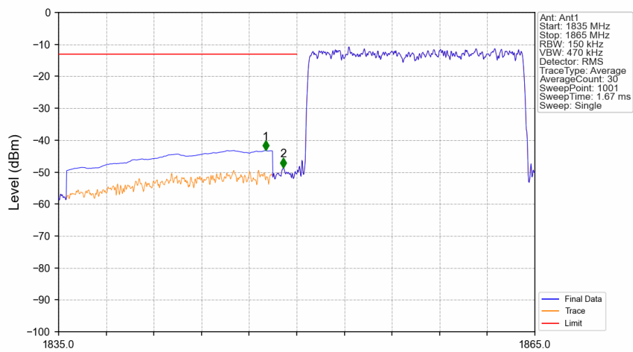
Band2_15MHz_16QAM_LCH_1857.5MHz_RB_75_0_NTNV
