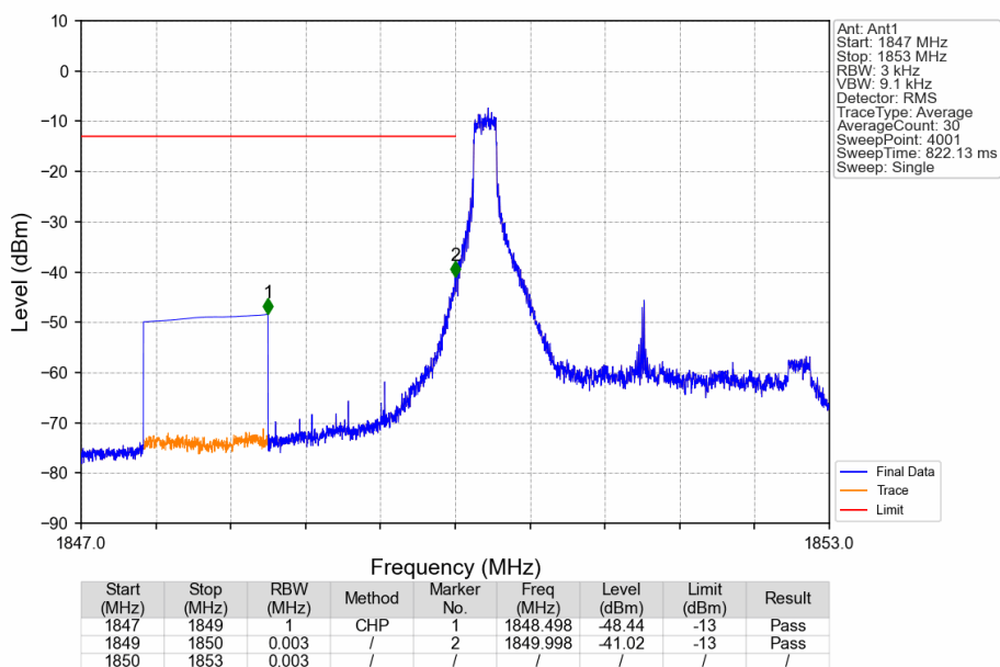
Band2_3MHz_16QAM_LCH_1851.5MHz_RB_1_0_NTNV
