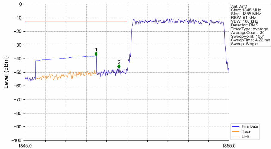
Band2_5MHz_16QAM_LCH_1852.5MHz_RB_25_0_NTNV
