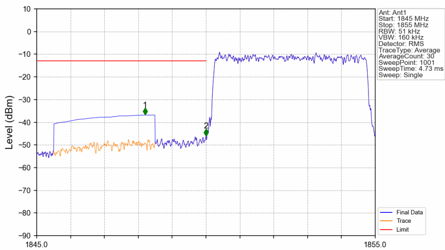
Band2_5MHz_QPSK_LCH_1852.5MHz_RB_25_0_NTNV
