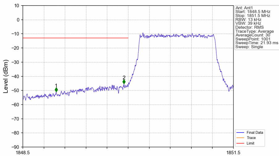
Band2_1.4MHz_QPSK_LCH_1850.7MHz_RB_6_0_NTNV
