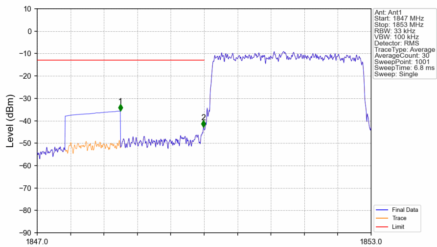
Band2_3MHz_QPSK_LCH_1851.5MHz_RB_15_0_NTNV
