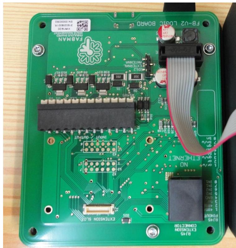
Logic Board connected
