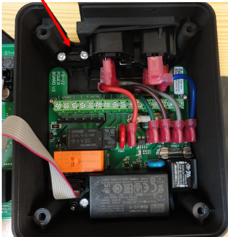
Power Board connected
