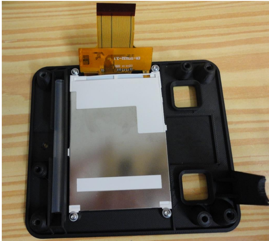
Display backside
