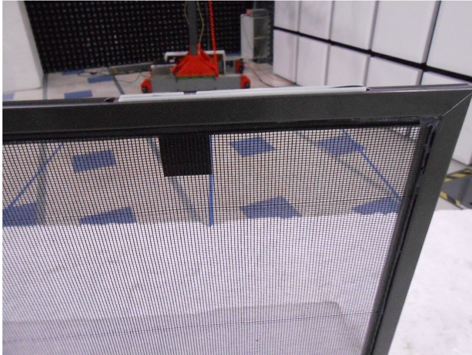
EUT installed in window Screen _ Final product
