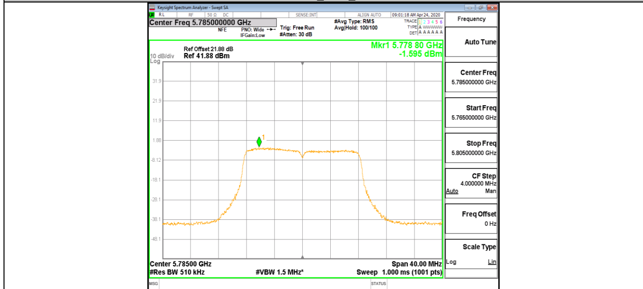
11A-CDD_Ant2_5785
