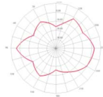
Efficiency:76.45
