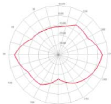
Efficiency:77.93
