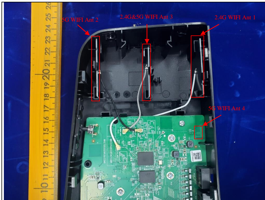
SR1021FS&SR1021F EUT-antenna
