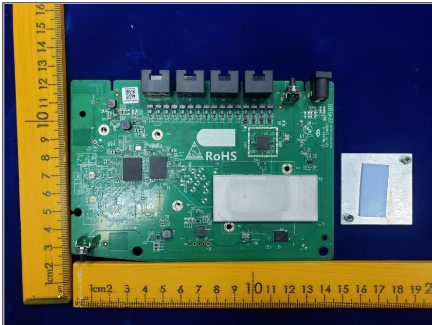
SR1021FS EUT-4
