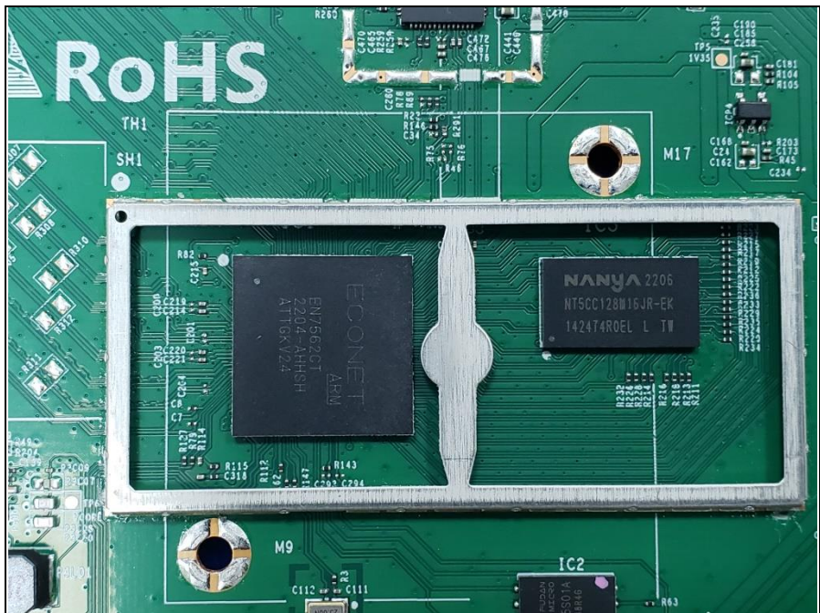
SR1021FS EUT-8
