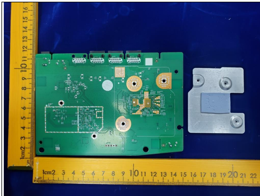
SR1021F EUT-11
