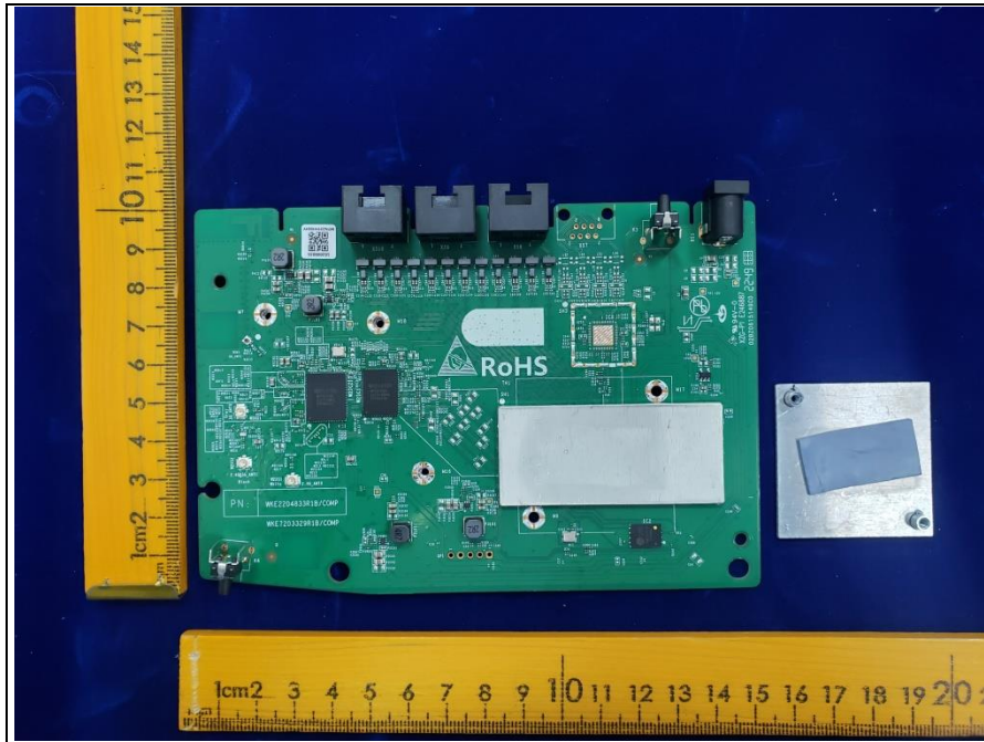
SR1021F EUT-4
