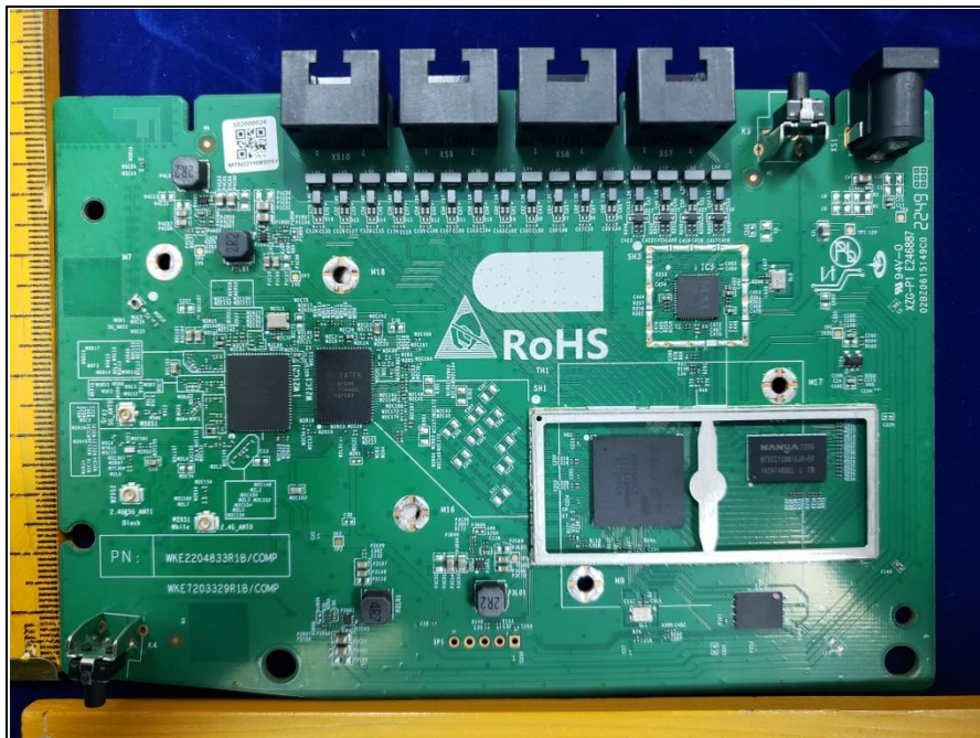
SR1021FS EUT-6
