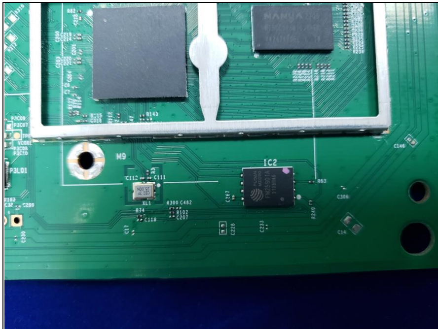
SR1021FS EUT-10
