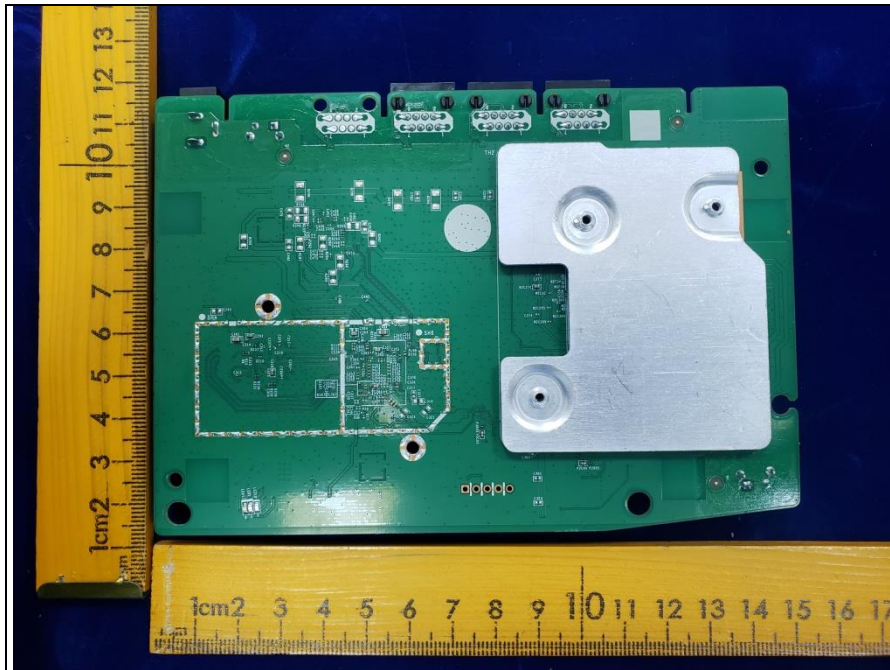
SR1021F EUT-10
