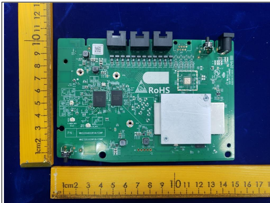
SR1021F EUT-3
