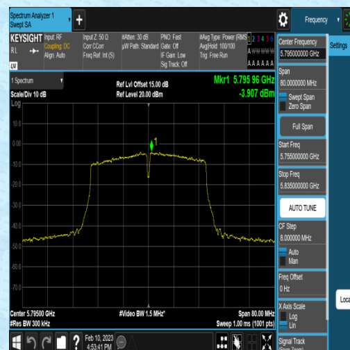
11N40MIMO-Ant2-5795--6.45-0.32-2.22-0.00
