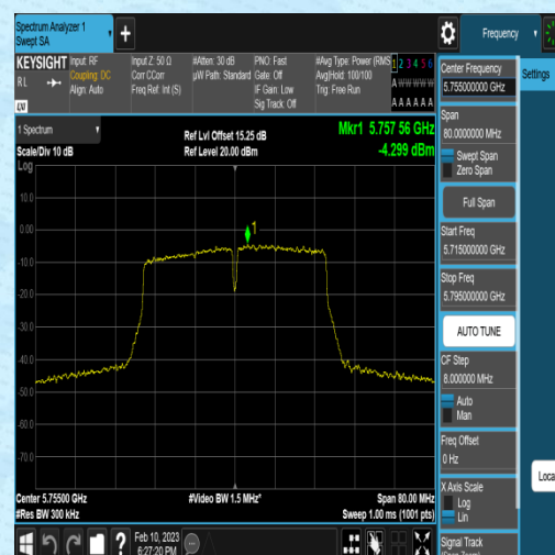
11AC40MIMO-Ant2-5755--7.10-0.58-2.22-0.00
