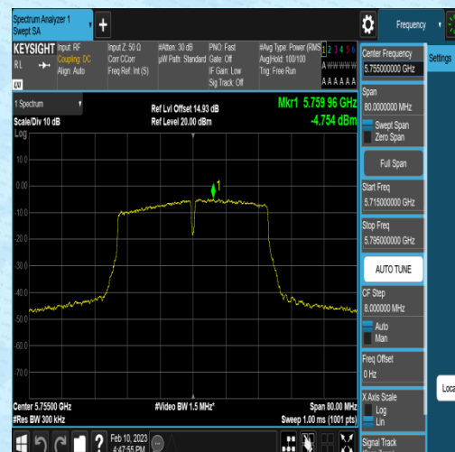
11N40MIMO-Ant2-5755--7.23-0.26-2.22-0.00
