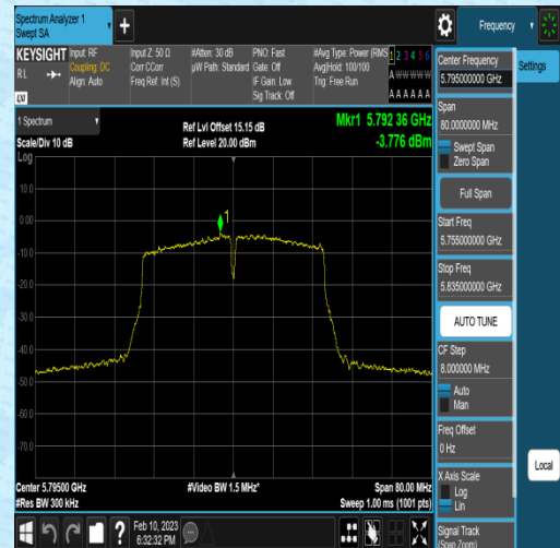
11AC40MIMO-Ant2-5795--6.47-0.47-2.22-0.00
