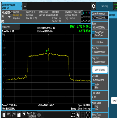
11AC80MIMO-Ant1-5775--10.02-0.83-2.22-0.00
