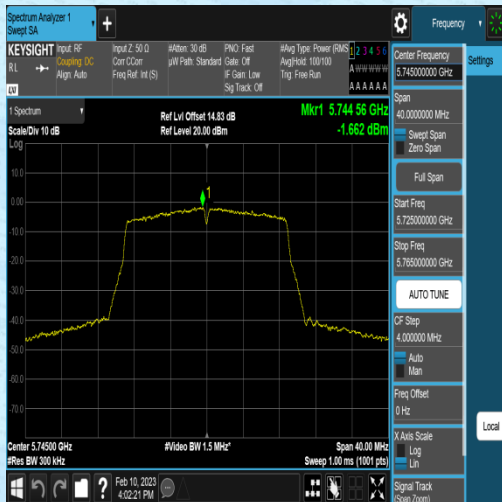
11N20MIMO-Ant2-5745--4.01-0.13-2.22-0.00
