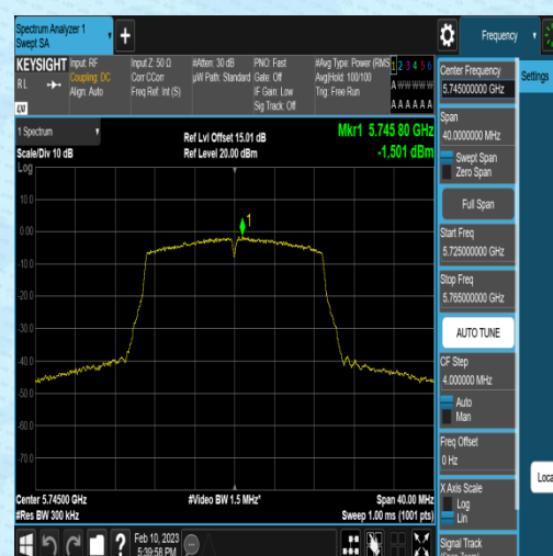
11AC20MIMO-Ant2-5745--4.03-0.31-2.22-0.00
