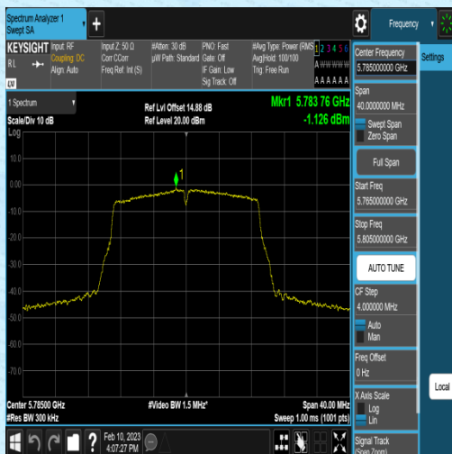
11N20MIMO-Ant2-5785--3.52-0.17-2.22-0.00
