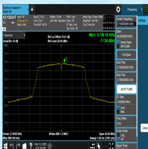
11AC20MIMO-Ant1-5745--3.65-0.31-2.22-0.00
