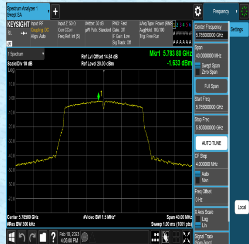
11N20MIMO-Ant1-5785--3.98-0.13-2.22-0.00
