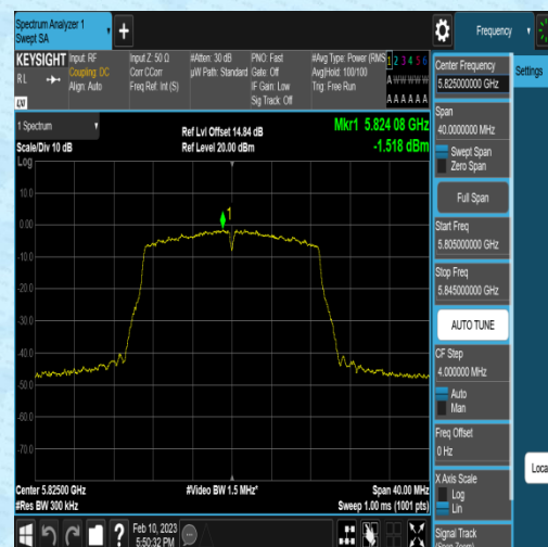
11AC20MIMO-Ant2-5825--3.99-0.25-2.22-0.00
