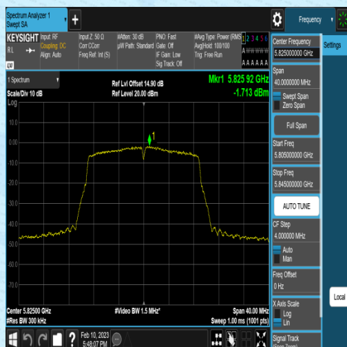
11AC20MIMO-Ant1-5825--4.24-0.31-2.22-0.00
