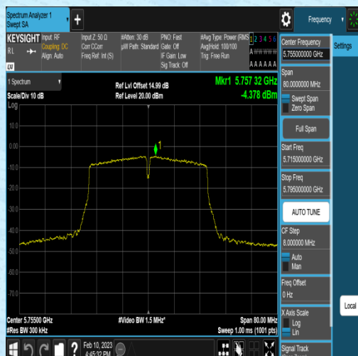
11N40MIMO-Ant1-5755--6.92-0.32-2.22-0.00
