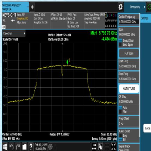
11AC40MIMO-Ant1-5795--7.16-0.46-2.22-0.00
