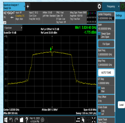
11N20MIMO-Ant1-5825--4.13-0.13-2.22-0.00
