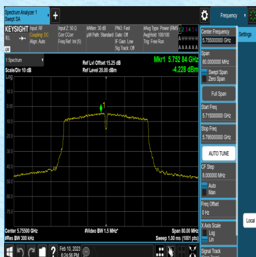
11AC40MIMO-Ant1-5755--7.03-0.58-2.22-0.00
