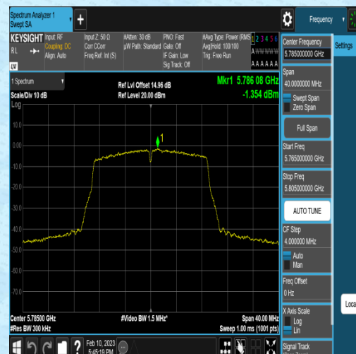
11AC20MIMO-Ant2-5785--3.82-0.25-2.22-0.00
