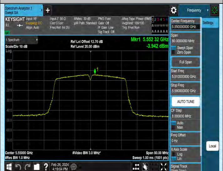
11AC40SISO-Ant2-5550-PASS
