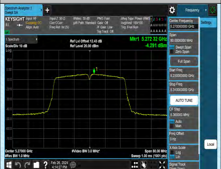
11AC40SISO-Ant2-5270-PASS
