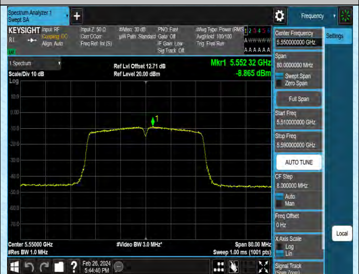
11N40MIMO-Ant2-5550-PASS
