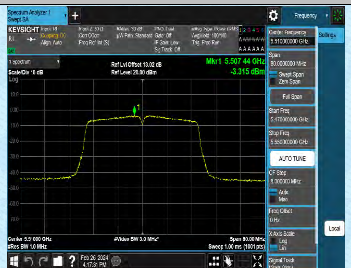
11AC40SISO-Ant2-5510-PASS
