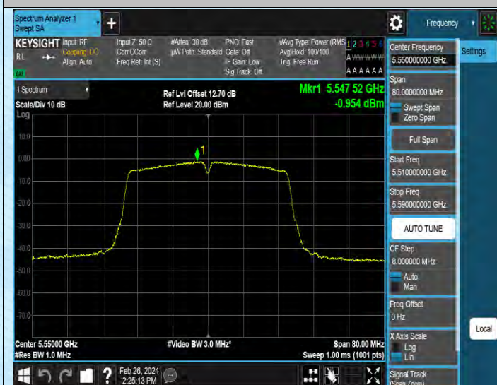
11AC40SISO-Ant1-5550-PASS
