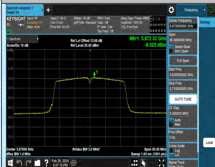
11N40MIMO-Ant1-5670-PASS
