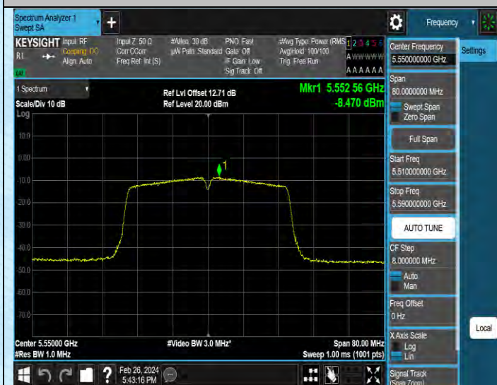
11N40MIMO-Ant1-5550-PASS
