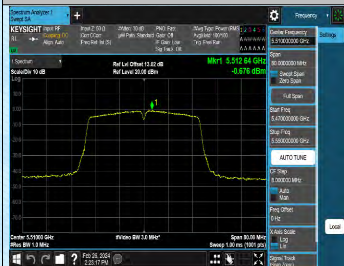
11AC40SISO-Ant1-5510-PASS
