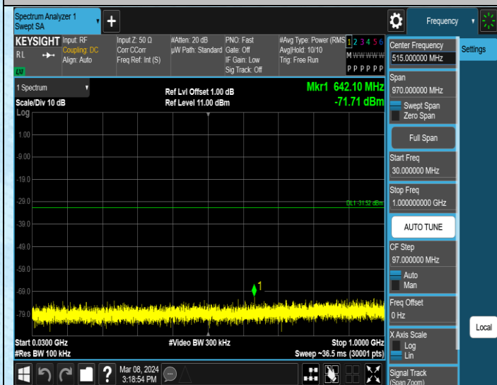
11AX20MIMO-Ant2-2437-30-1000-PASS
