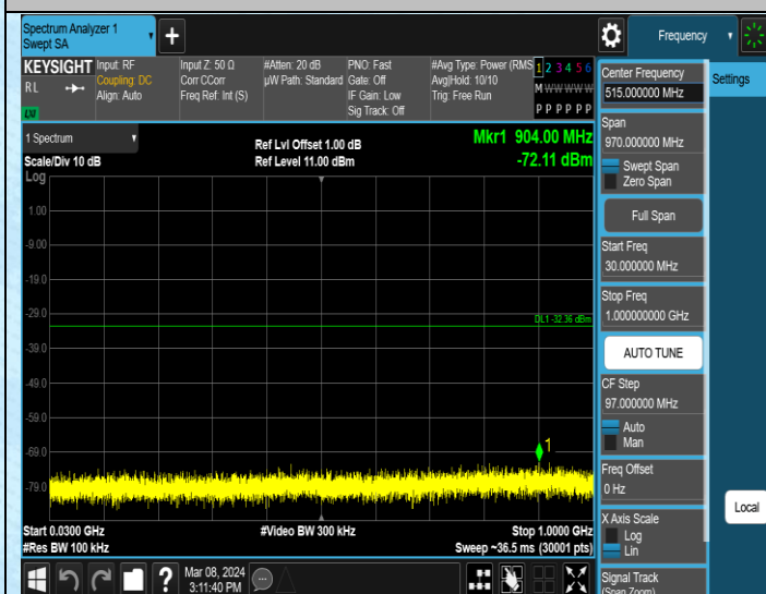
11N20MIMO-Ant2-2462-30~1000-PASS
