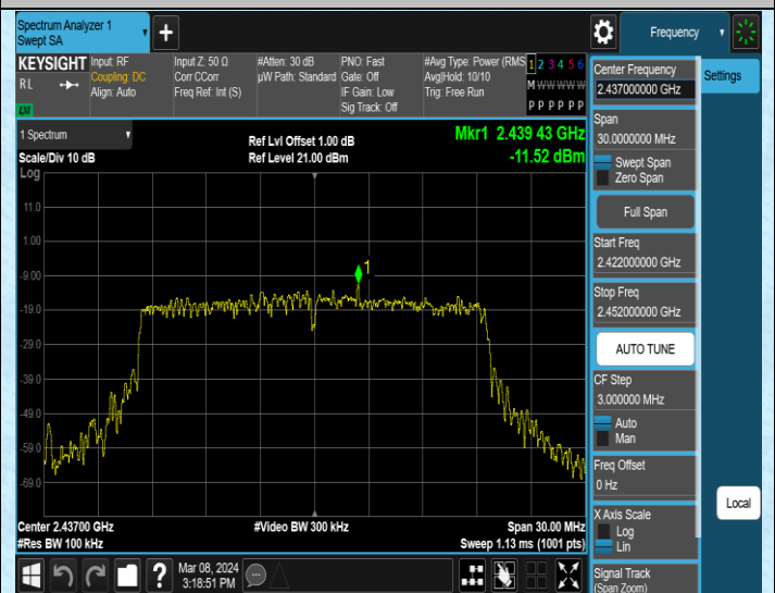
11AX20MIMO-Ant2-2437-0-Reference-PASS
