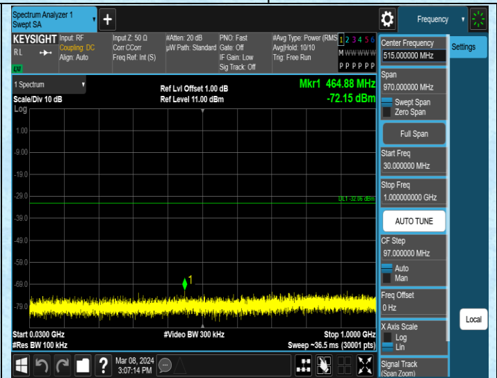
11N20MIMO-Ant1-2437-30~1000-PASS
