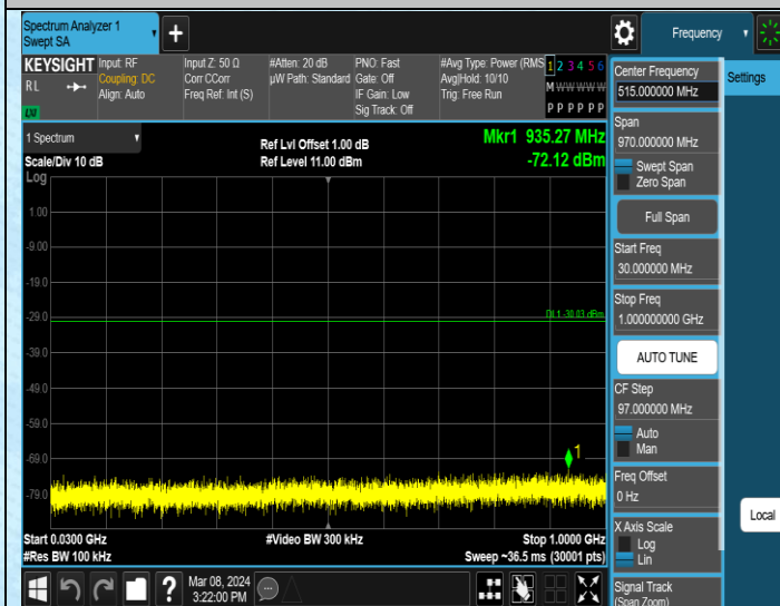
11AX20MIMO-Ant2-2462-30~1000-PASS
