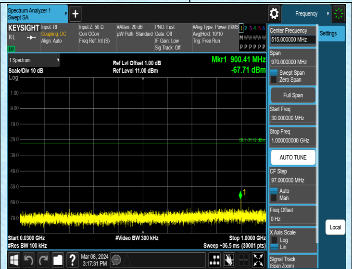
11AX20MIMO-Ant1-2437-30-1000-PASS
