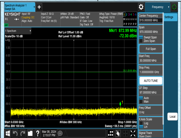
11N20SISO-Ant1-2437-30-1000-PASS
