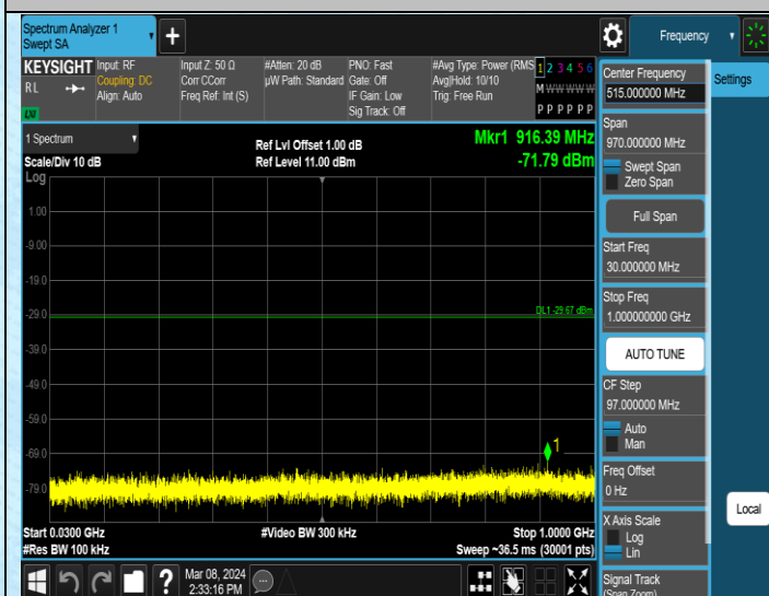
11G-Ant2-2437-30-1000-PASS
