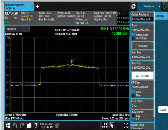
11AX80MIMO-Ant1-5775-PASS
