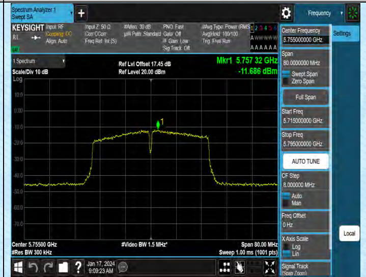
11AC40MIMO-Ant2-5755-PASS
