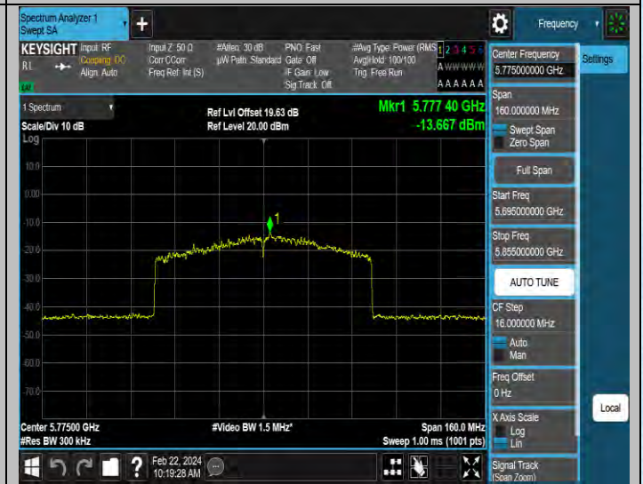
11AX80MIMO-Ant2-5775-PASS
