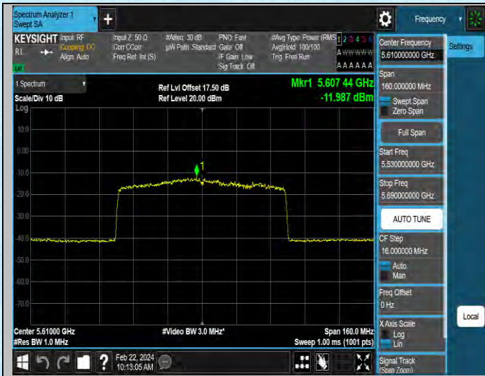
11AX80MIMO-Ant1-5610-PASS
