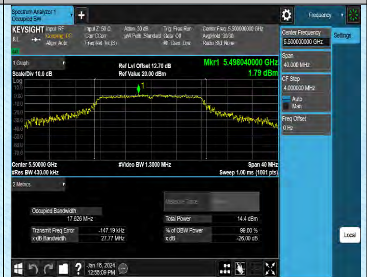
11A-Ant2-5500
