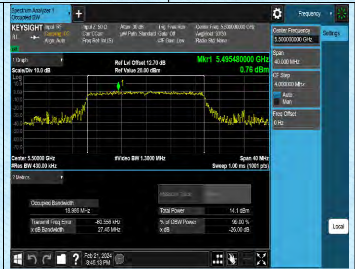
11AX20SISO-Ant2-5500
