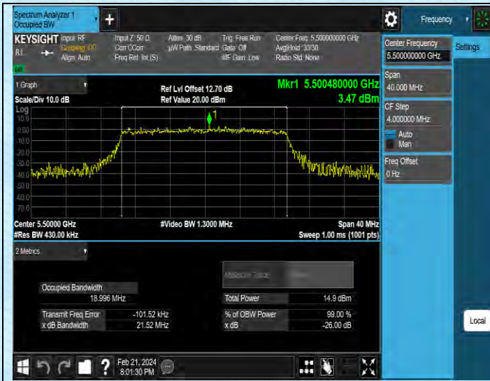
11AX20SISO-Ant1-5500
