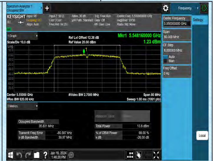
11N40SISO-Ant2-5550
