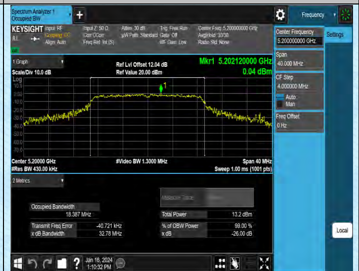
11N20SISO-Ant2-5200
