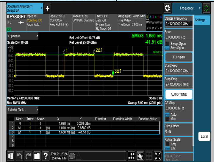
NTNV-11AX20MIMO-Ant2-2412
