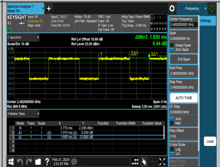
NTNV-11AX20MIMO-Ant2-2462
