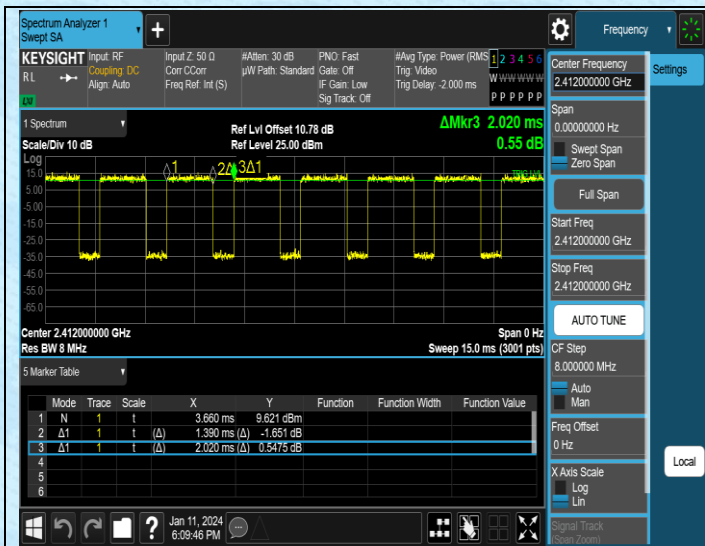
NTNV-11G-Ant1-2412
