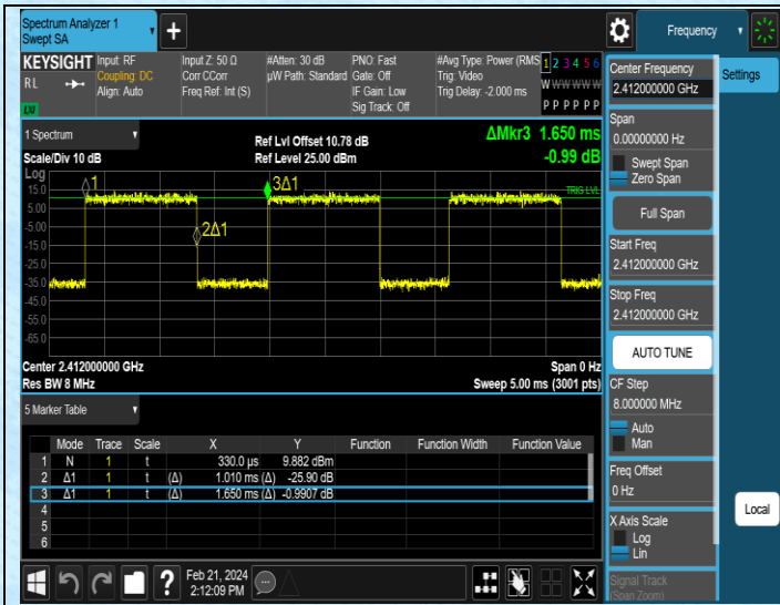
NTNV-11AX20SISO-Ant1-2412
