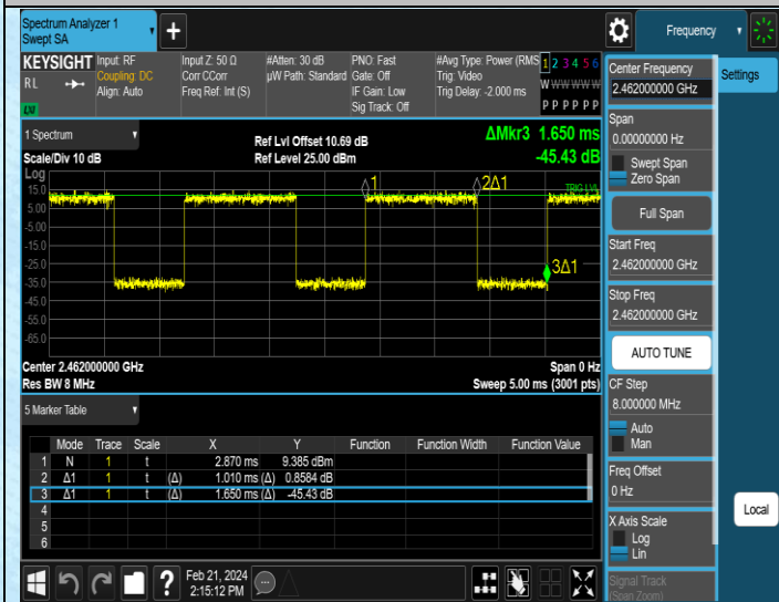
NTNV-11AX20SISO-Ant1-2462
