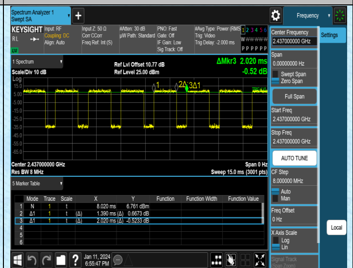
NTNV-11G-Ant2-2437
