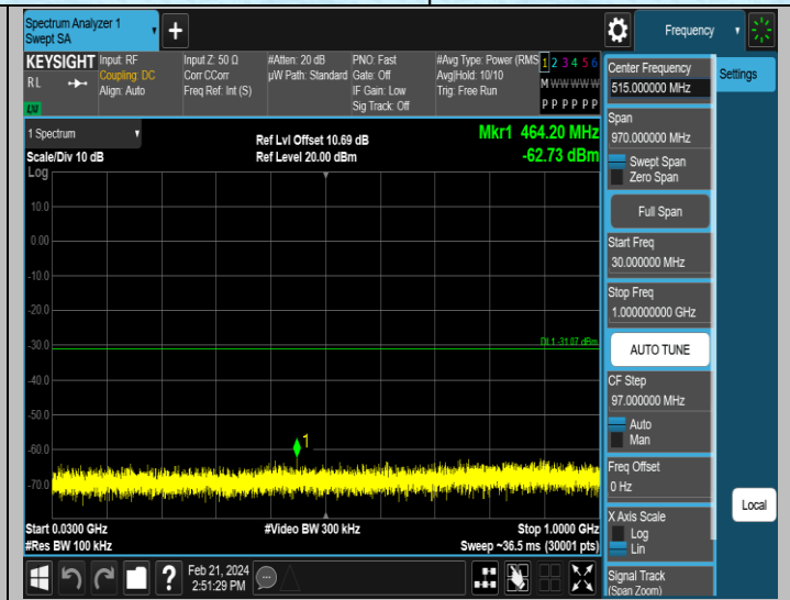
11AX20MIMO-Ant1-2462-30-1000-PASS
