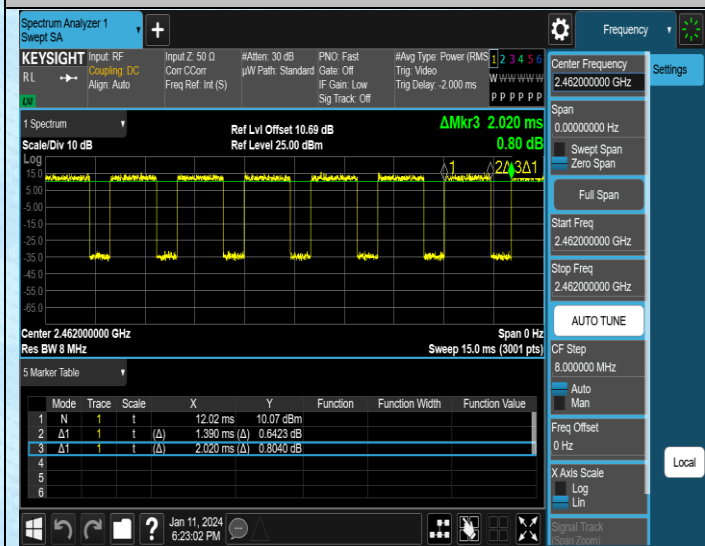
NTNV-11G-Ant1-2462
