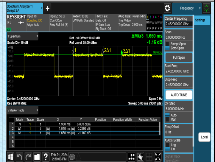
NTNV-11AX20SISO-Ant2-2462
