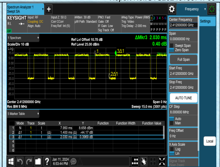
NTNV-11G-Ant2-2412
