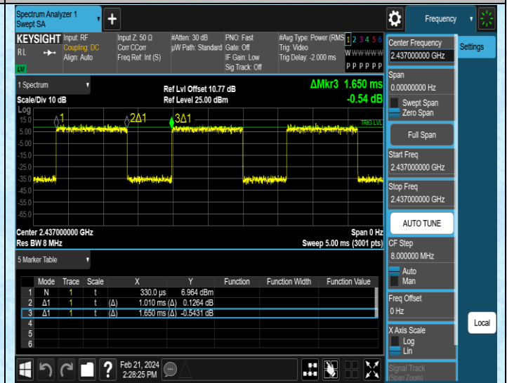
NTNV-11AX20SISO-Ant2-2437
