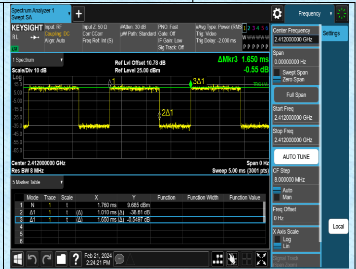
NTNV-11AX20SISO-Ant2-2412
