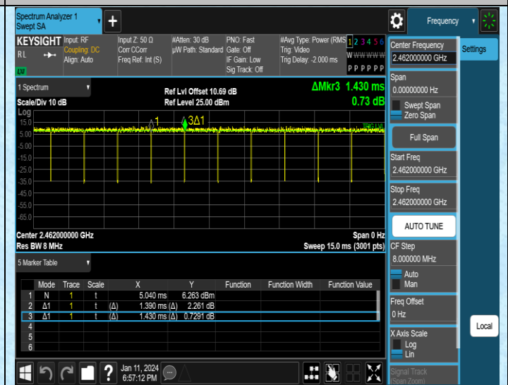
NTNV-11G-Ant2-2462
