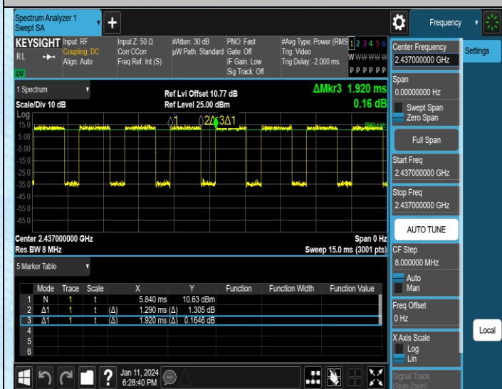
NTNV-11N20SISO-Ant1-2437
