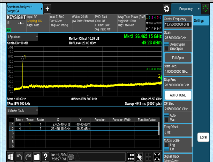
11N20MIMO-Ant2-2462-1000~26500-PASS
