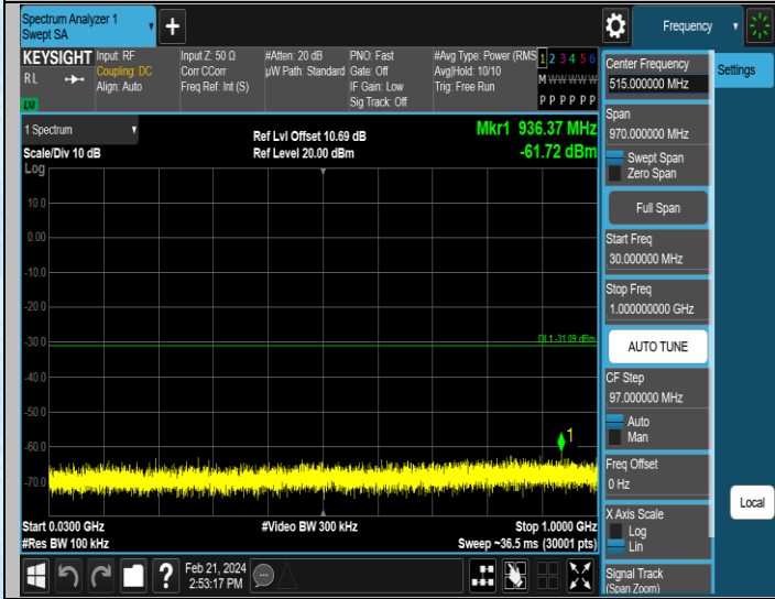
11AX20MIMO-Ant2-2462-30-1000-PASS
