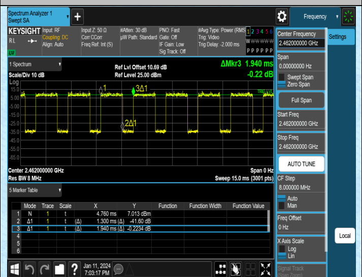
NTNV-11N20SISO-Ant2-2462
