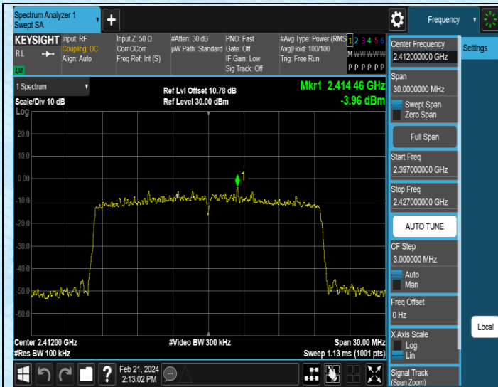
11AX20SISO-Ant1-2412-0~Reference-PASS
