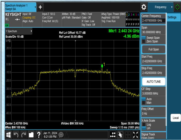
11G-Ant1-2437-0~Reference-PASS
