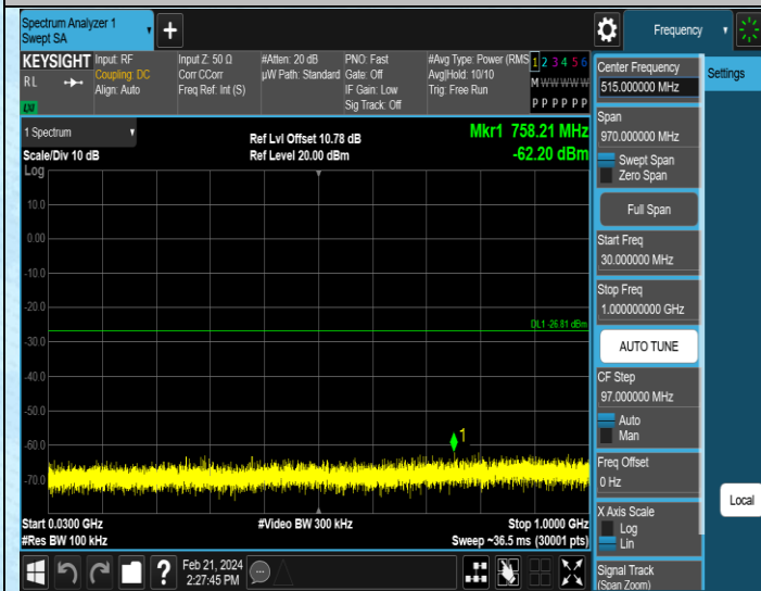
11AX20SISO-Ant2-2412-30~1000-PASS
