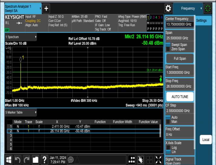
11N20MIMO-Ant2-2412-1000~26500-PASS
