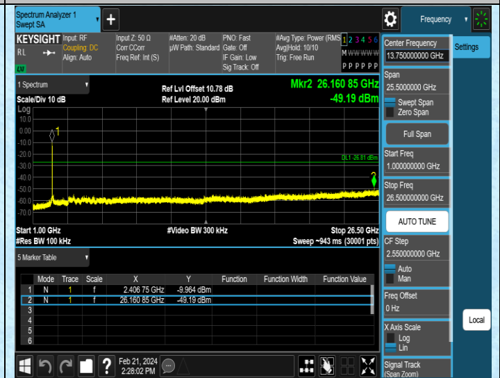
11AX20SISO-Ant2-2412-1000~26500-PASS
