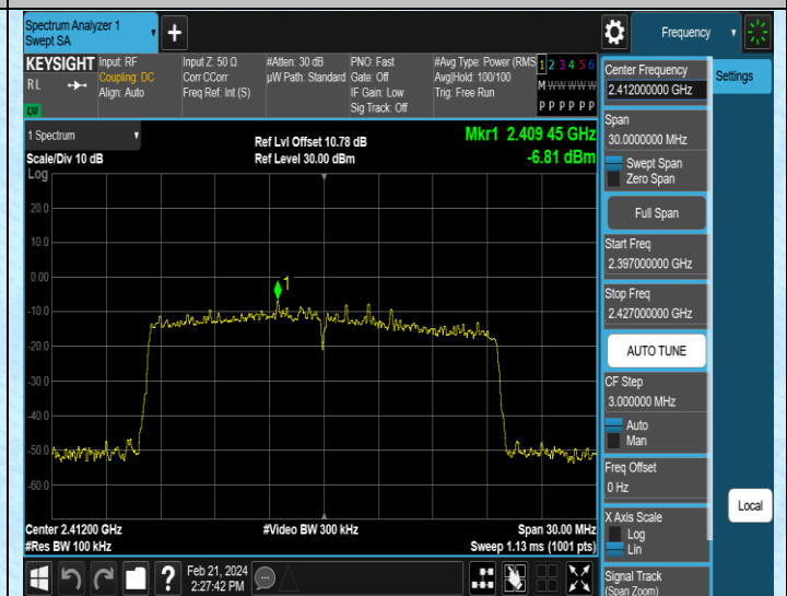
11AX20SISO-Ant2-2412-0~Reference-PASS
