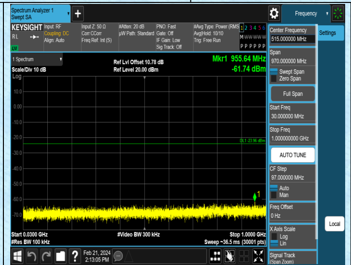
11AX20SISO-Ant1-2412-30~1000-PASS
