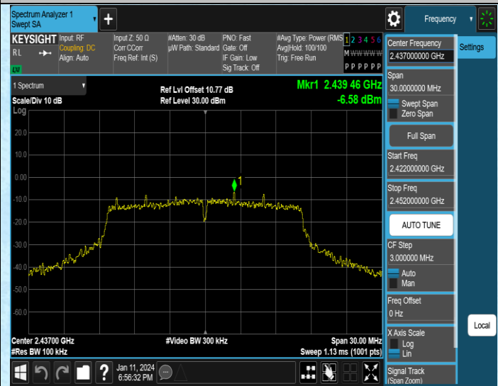
11G-Ant2-2437-0~Reference-PASS
