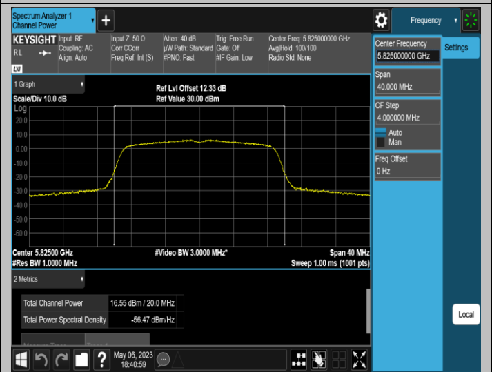
11N20SISO-Ant2-5825
