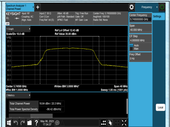
11A-Ant2-5745
