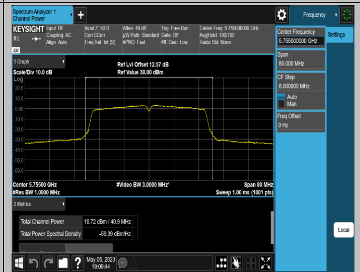
11AC40SISO-Ant2-5755
