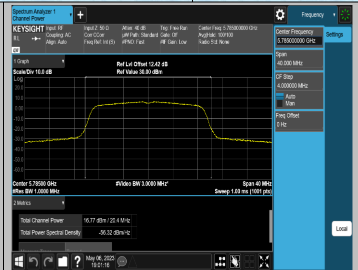
11AC20SISO-Ant2-5785
