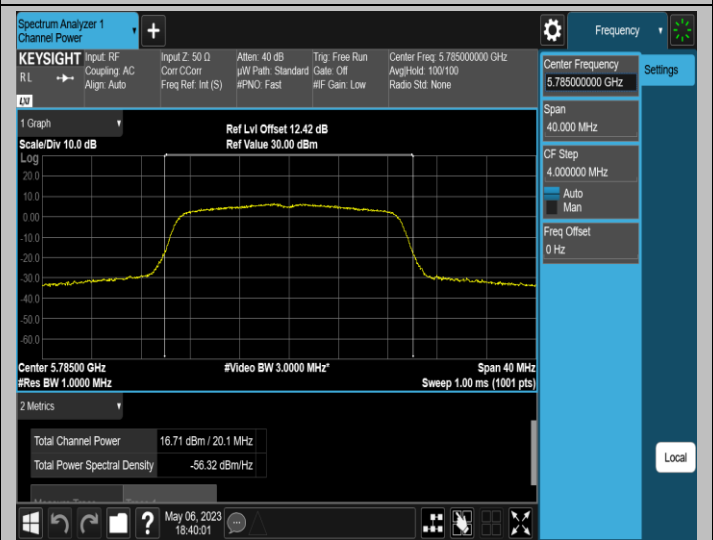
11N20SISO-Ant2-5785
