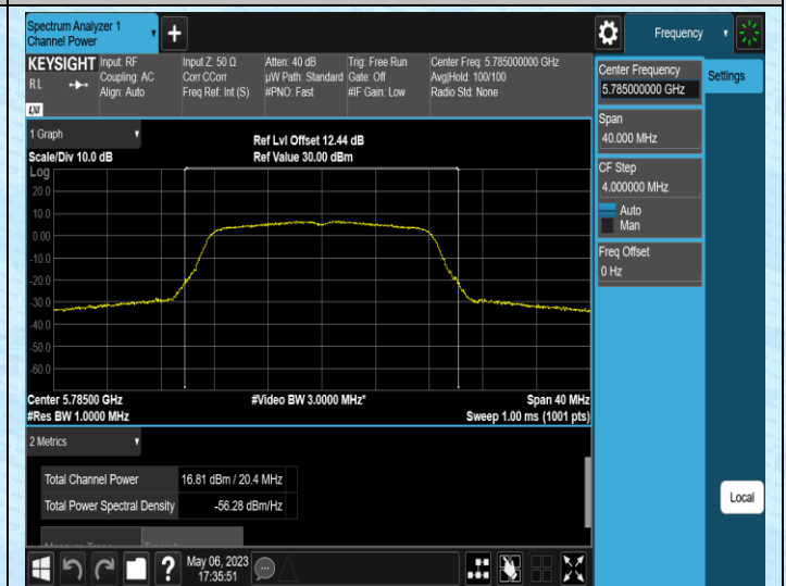
11A-Ant2-5785
