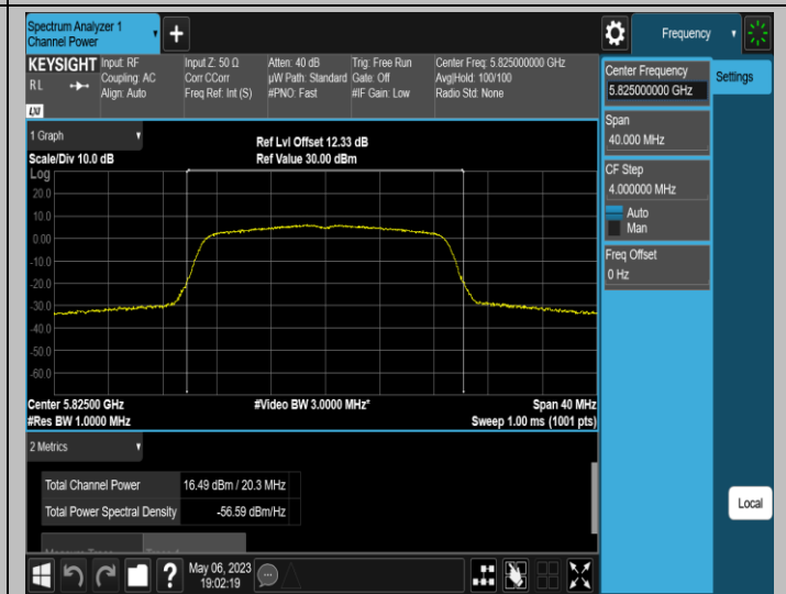
11AC20SISO-Ant2-5825
