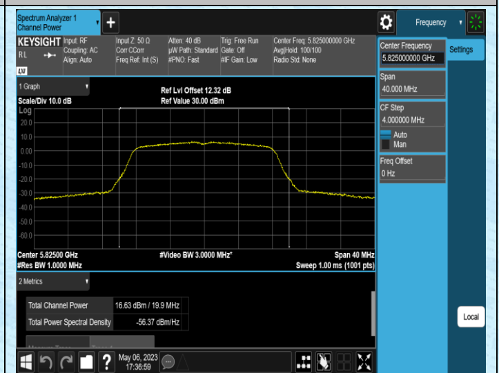
11A-Ant2-5825
