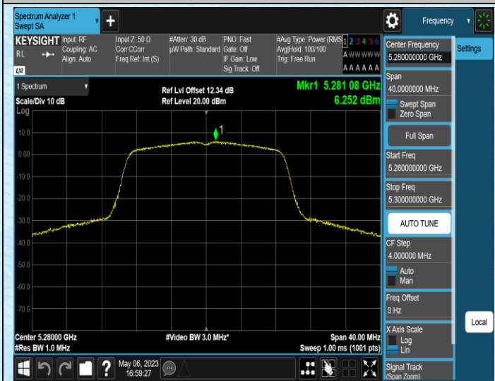
11AC20SISO-Ant1-5280
