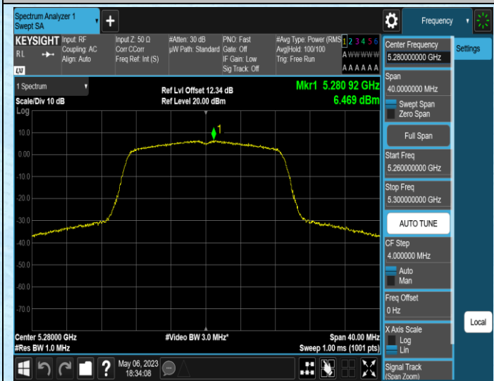
11N20SISO-Ant2-5280
