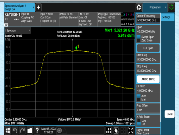
11AC20SISO-Ant1-5320
