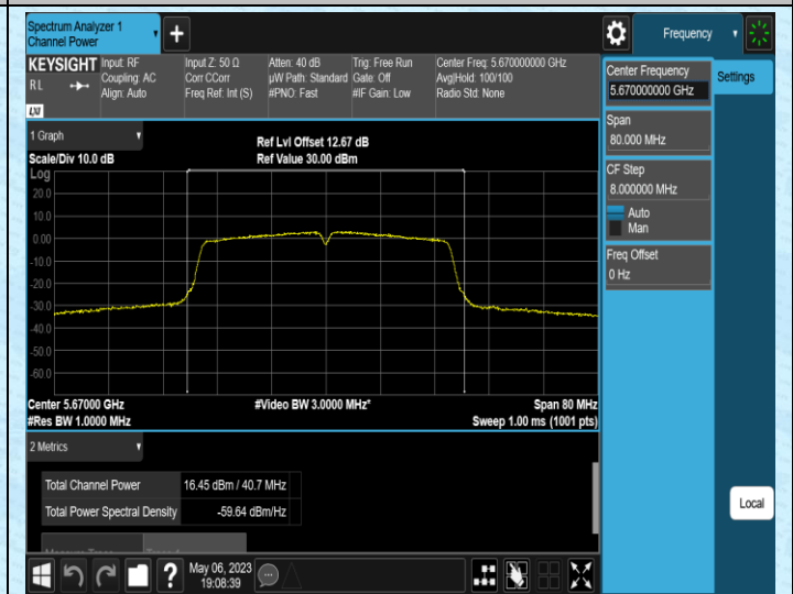
11AC40SISO-Ant2-5670
