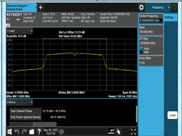
11AC40SISO-Ant2-5550
