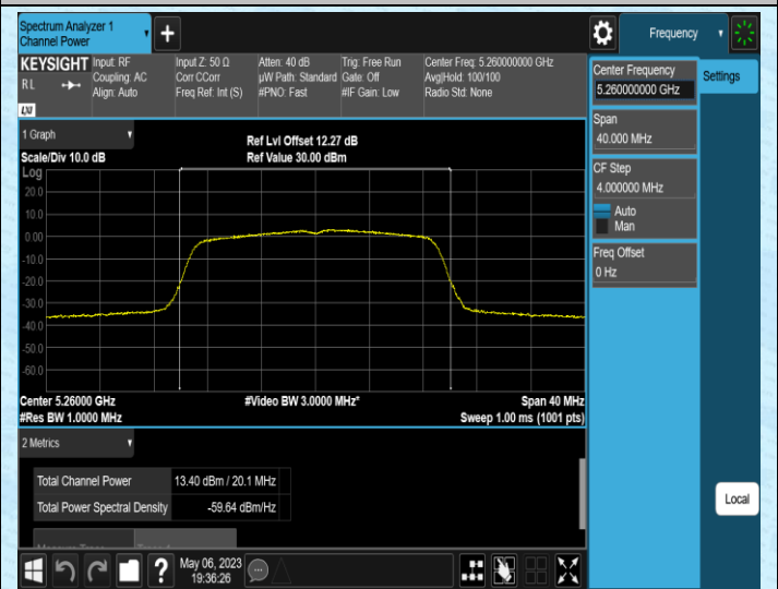
11N20MIMO-Ant2-5260
