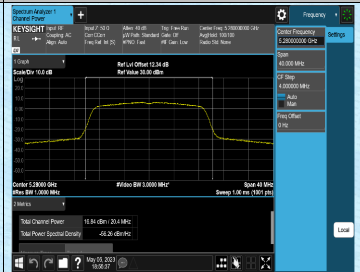
11AC20SISO-Ant2-5280
