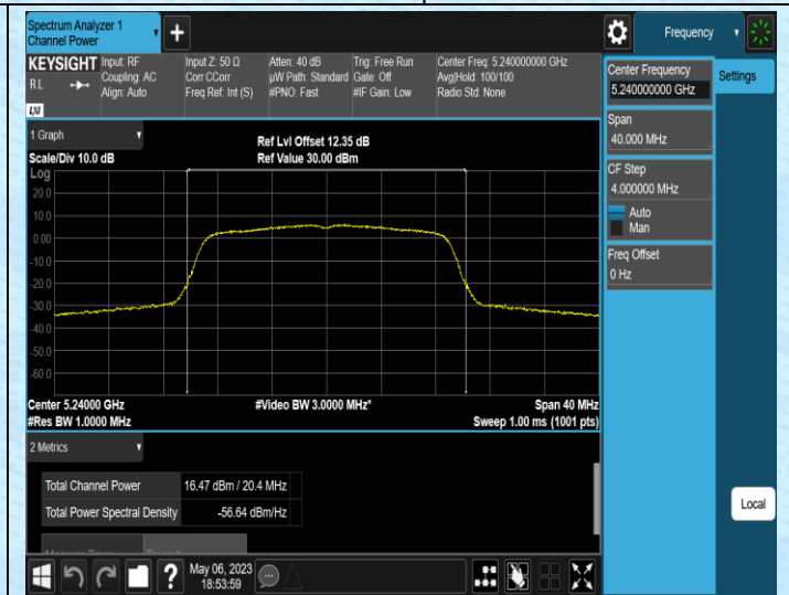
11AC20SISO-Ant2-5240
