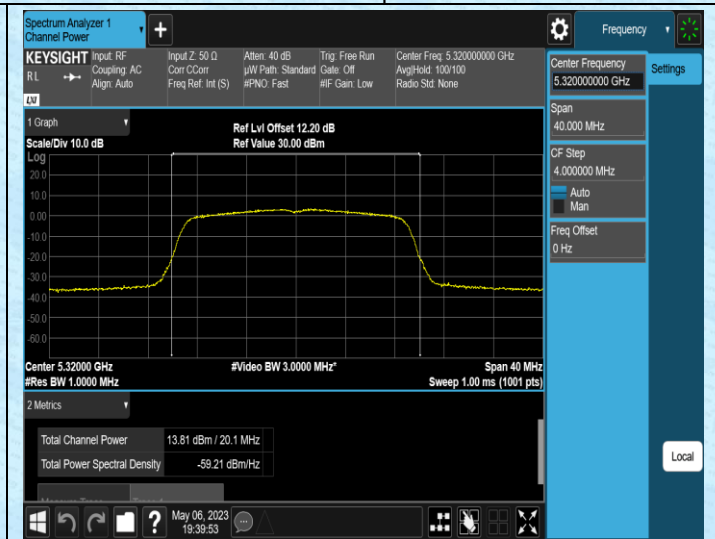
11N20MIMO-Ant2-5320
