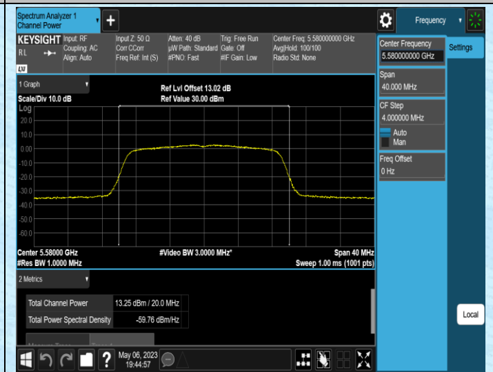
11N20MIMO-Ant2-5580
