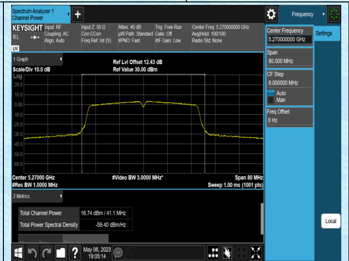
11AC40SISO-Ant2-5270
