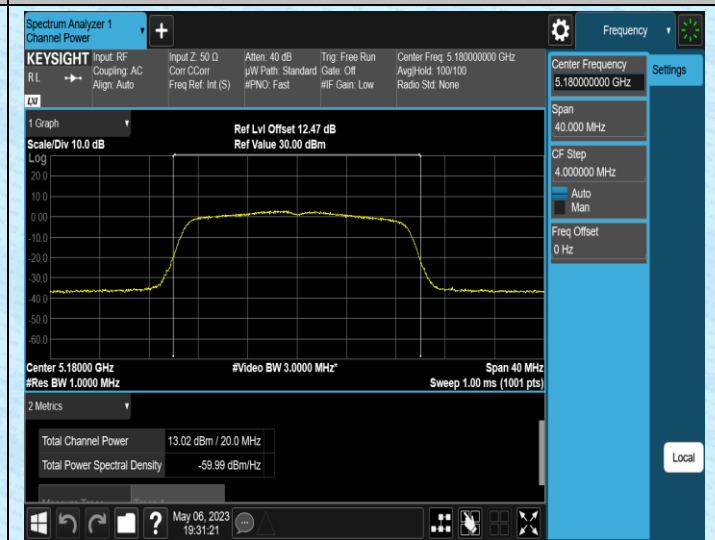
11N20MIMO-Ant2-5180
