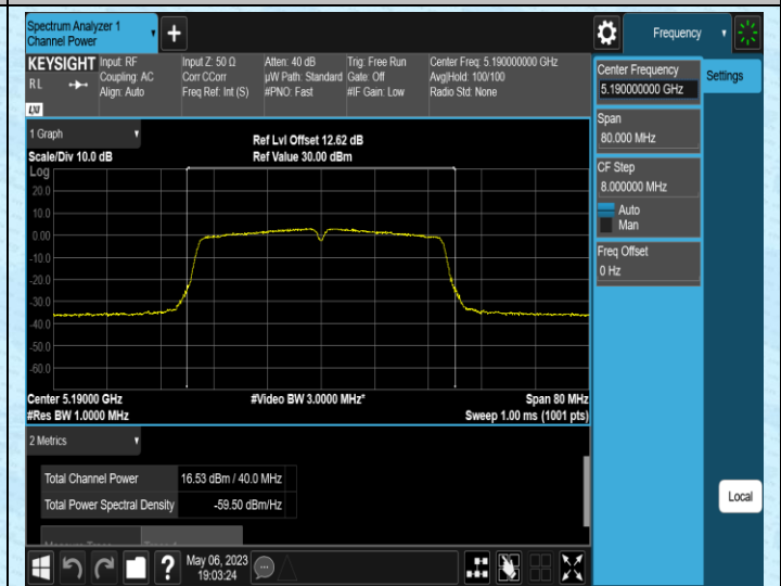
11AC40SISO-Ant2-5190
