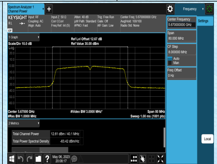
11N40MIMO-Ant2-5670
