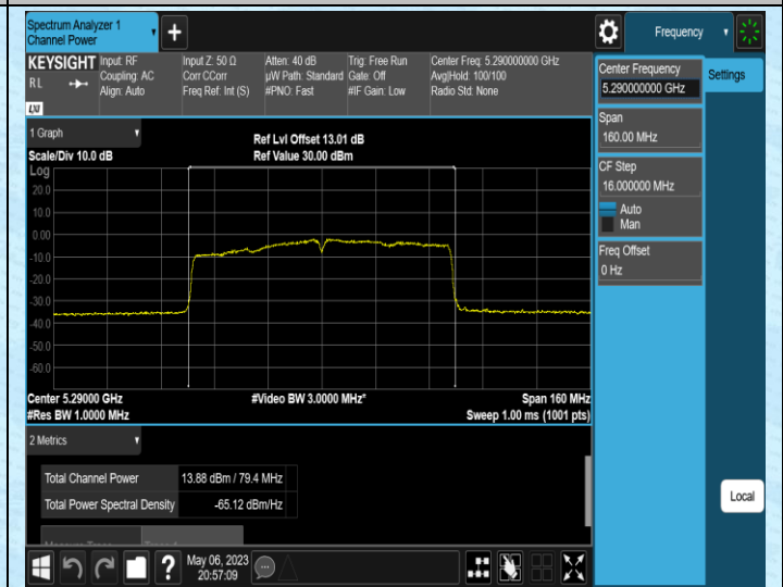
11AC80MIMO-Ant2-5290
