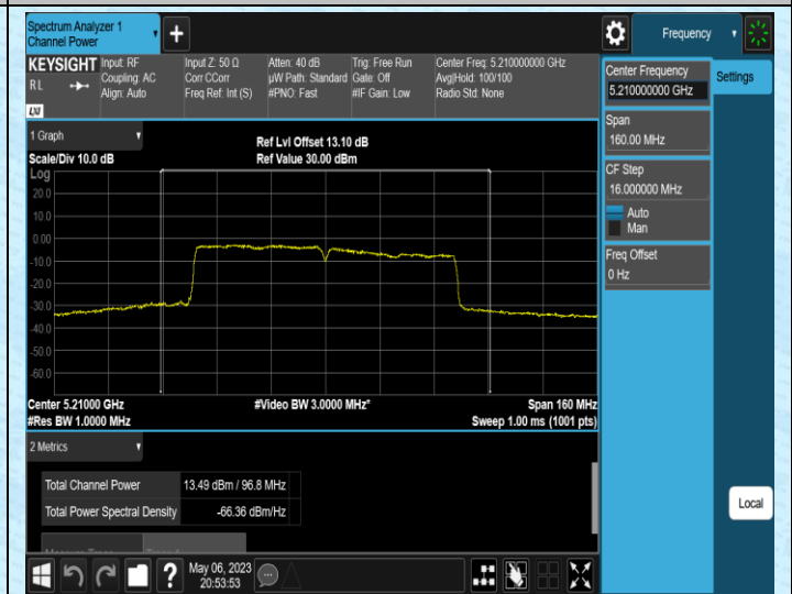
11AC80MIMO-Ant2-5210
