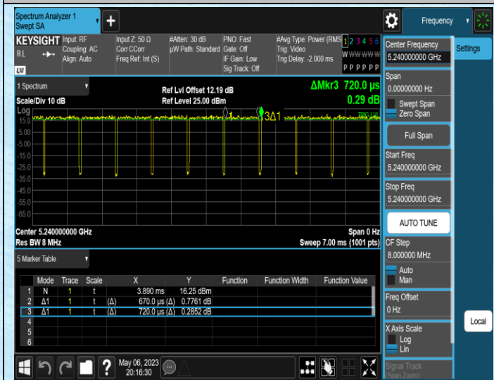
NTNV-11AC20MIMO-Ant1-5240
