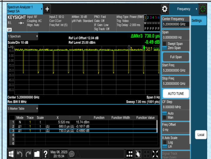
NTNV-11AC20MIMO-Ant2-5200
