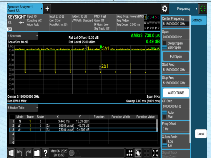
NTNV-11AC20MIMO-Ant2-5180
