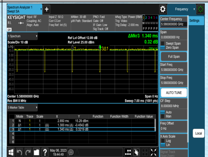
NTNV-11N20MIMO-Ant2-5580
