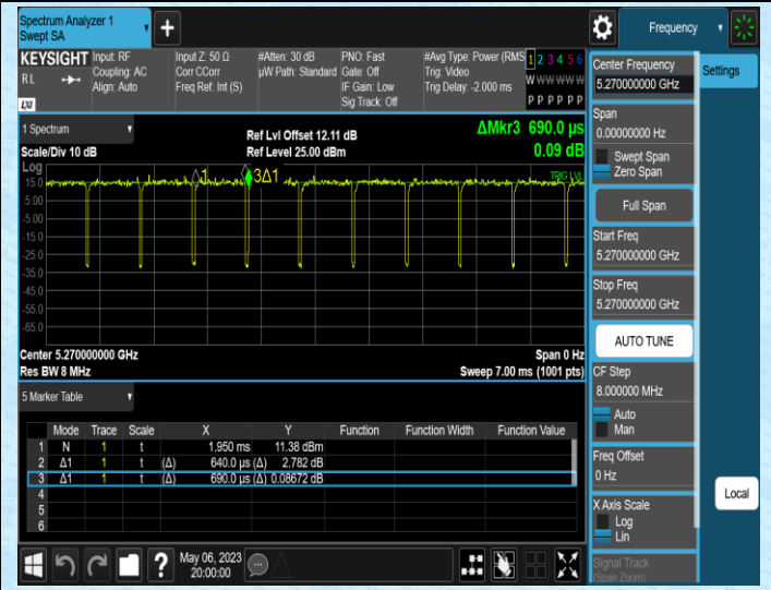
NTNV-11N40MIMO-Ant2-5270
