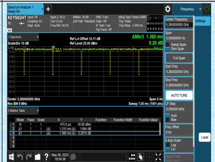
NTNV-11AC20SISO-Ant2-5260
