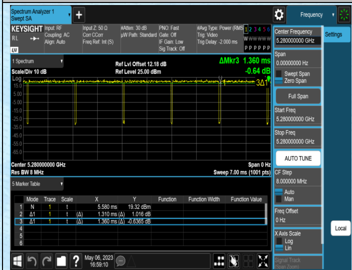
NTNV-11AC20SISO-Ant1-5280
