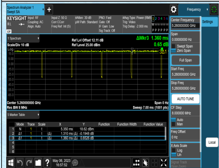
NTNV-11AC20SISO-Ant1-5260
