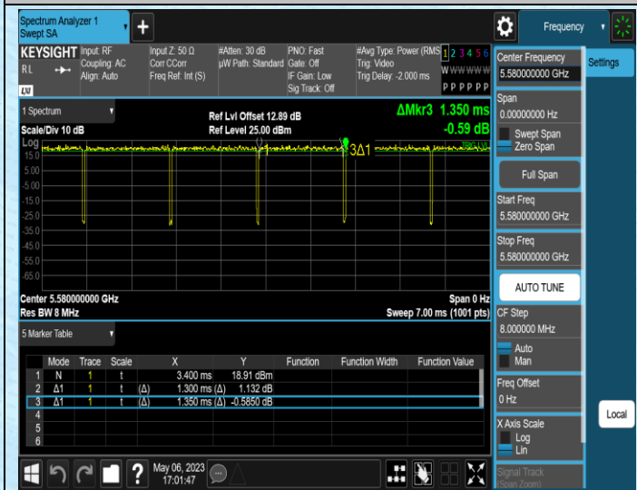
NTNV-11AC20SISO-Ant1-5580
