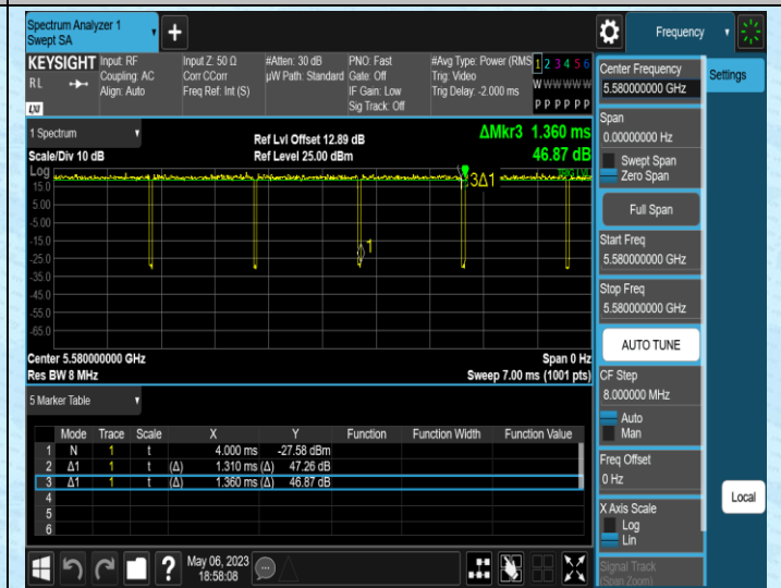
NTNV-11AC20SISO-Ant2-5580
