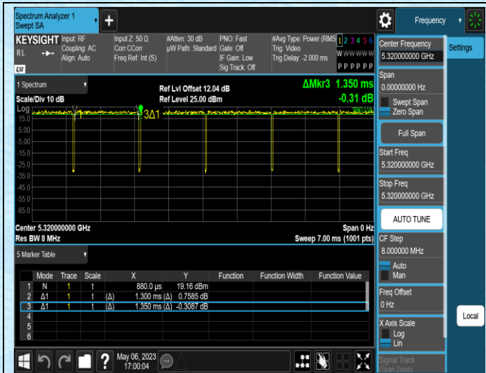
NTNV-11AC20SISO-Ant1-5320
