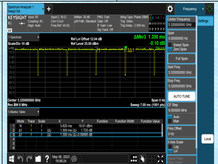
NTNV-11AC20SISO-Ant2-5320
