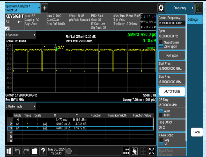
NTNV-11N40MIMO-Ant2-5190
