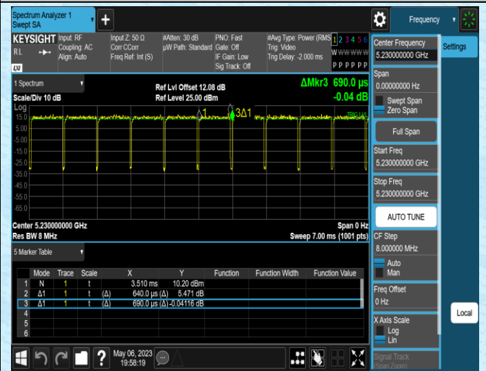
NTNV-11N40MIMO-Ant2-5230
