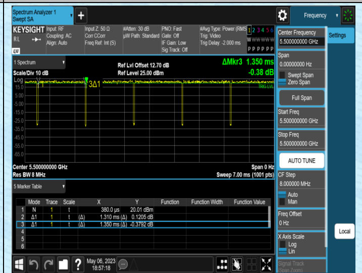
NTNV-11AC20SISO-Ant2-5500
