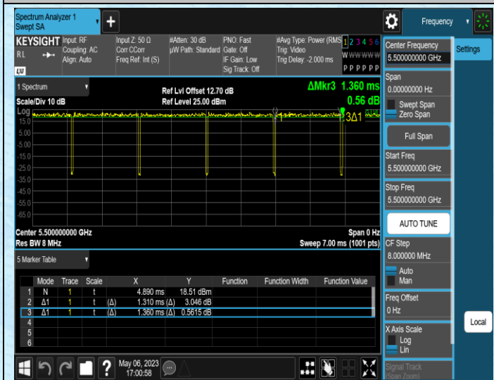
NTNV-11AC20SISO-Ant1-5500
