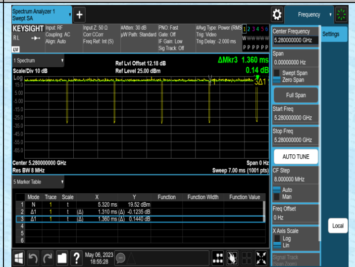
NTNV-11AC20SISO-Ant2-5280
