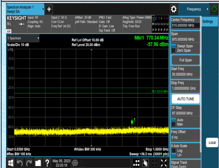
11N40SISO-Ant2-2452-30~1000
