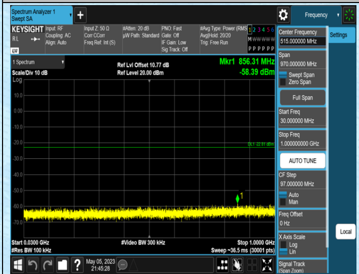
11N20SISO-Ant2-2437-30~1000
