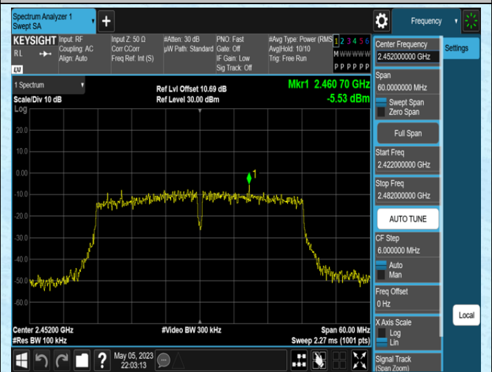
11N40SISO-Ant2-2452-0~Reference
