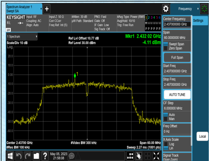
11N40SISO-Ant2-2437-0~Reference
