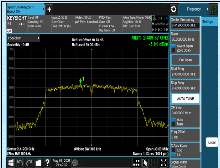
11N20SISO-Ant2-2412-0~Reference
