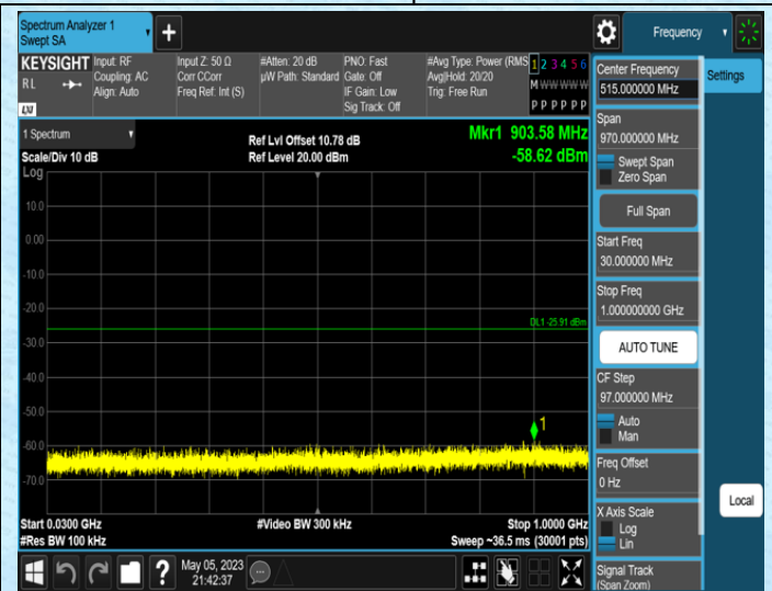
11N20SISO-Ant2-2412-30~1000
