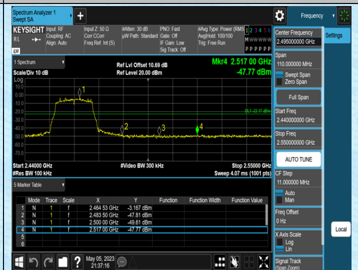
11G-Ant2-2462
