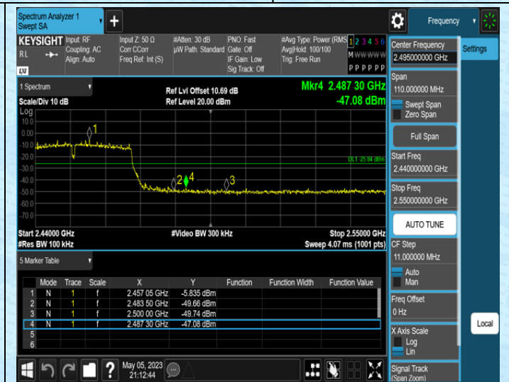
11N40SISO-Ant1-2452
