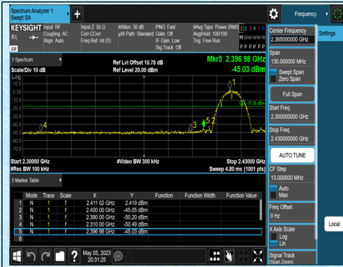
11B-Ant1-2412
