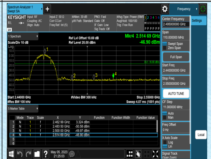
11B-Ant2-2462
