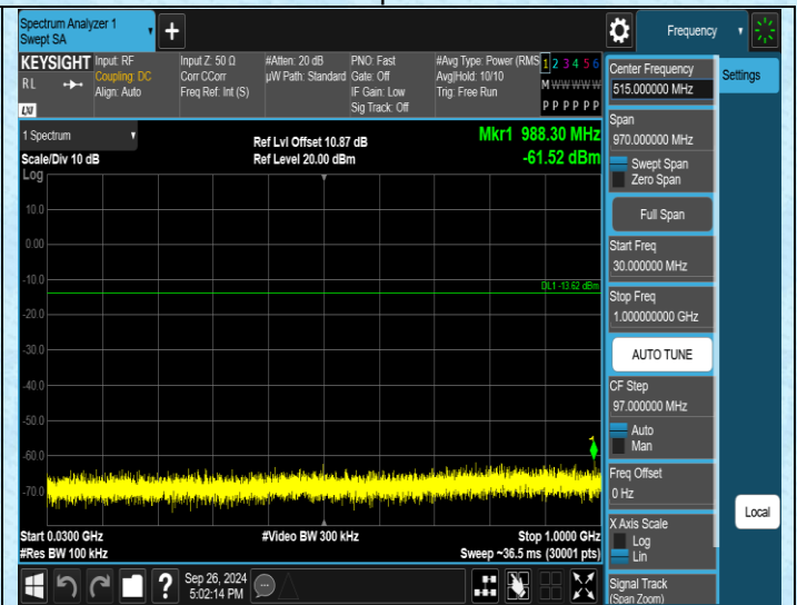
3DH5-Ant1-2480-30~1000-PASS
