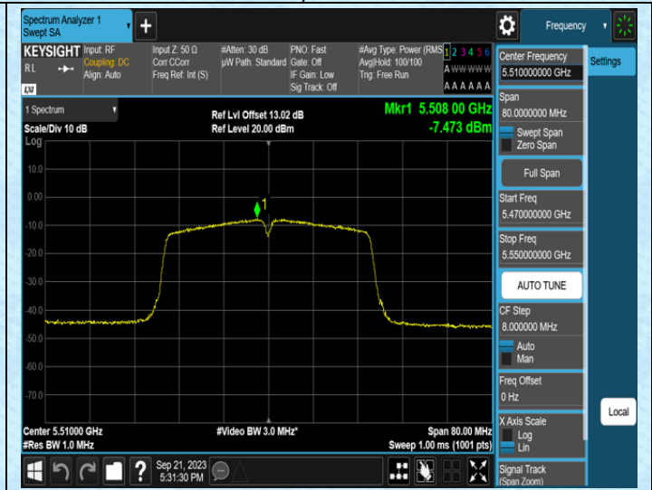
11AC40MIMO-Ant1-5510
