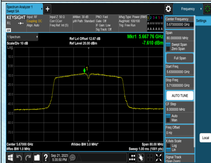
11AC40MIMO-Ant0-5670
