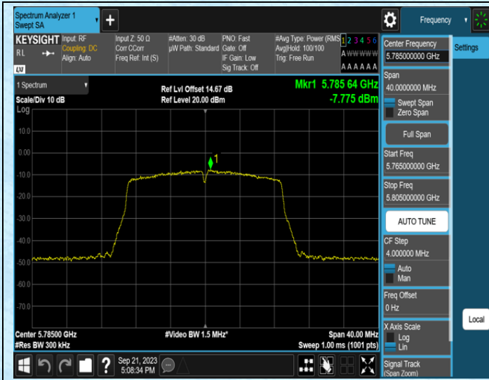
11AC20MIMO-Ant0-5785
