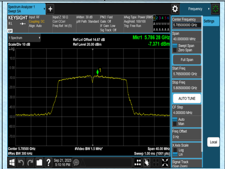
11AC20MIMO-Ant1-5785
