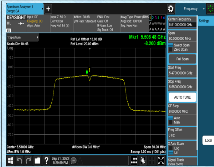
11AC40MIMO-Ant0-5510
