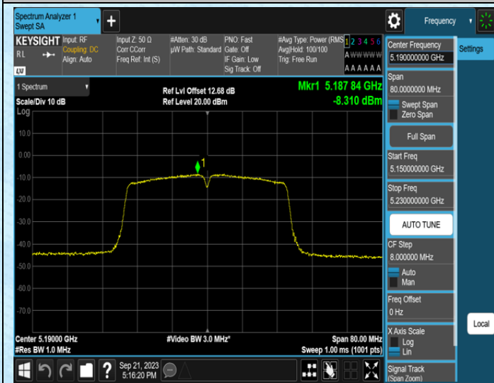
11AC40MIMO-Ant0-5190
