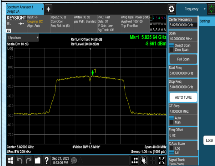
11AC20MIMO-Ant0-5825
