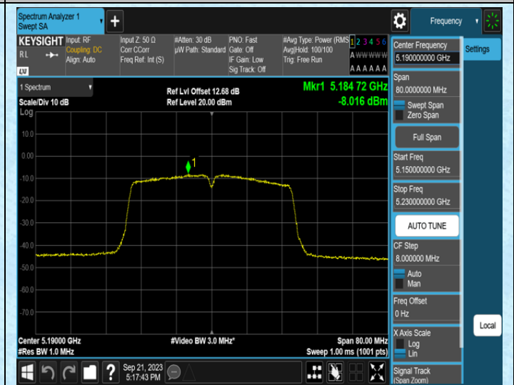
11AC40MIMO-Ant1-5190
