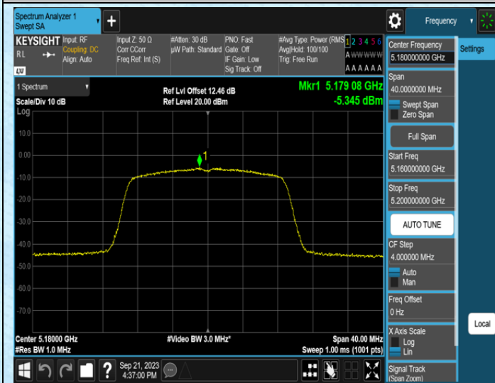
11AC20MIMO-Ant0-5180
