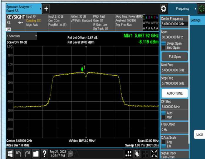
11N40MIMO-Ant0-5670
