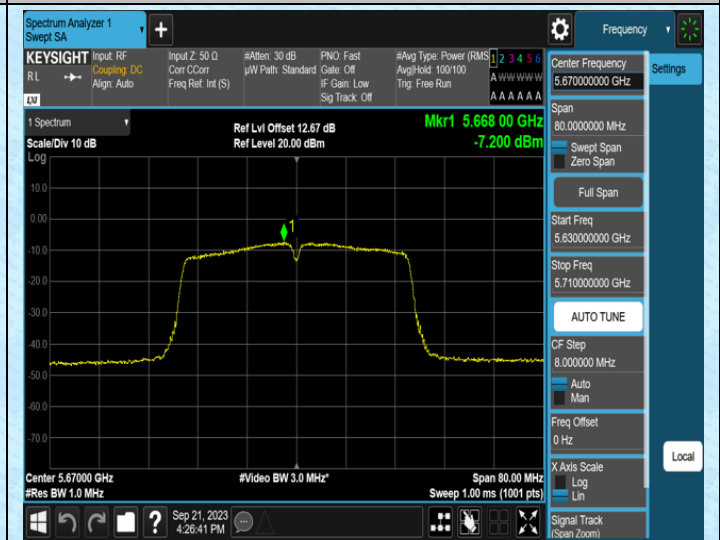
11N40MIMO-Ant1-5670
