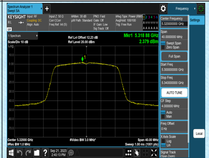
11AC20SISO-Ant1-5320
