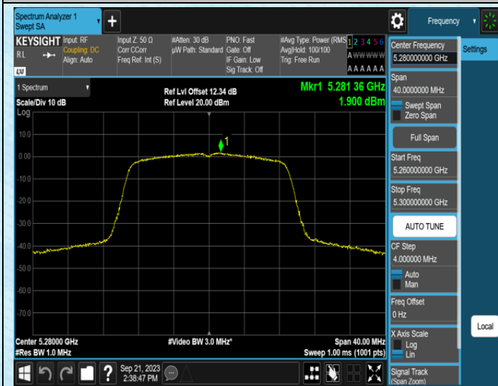
11AC20SISO-Ant1-5280
