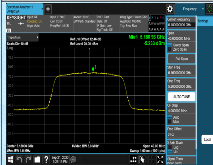
11N20MIMO-Ant0-5180
