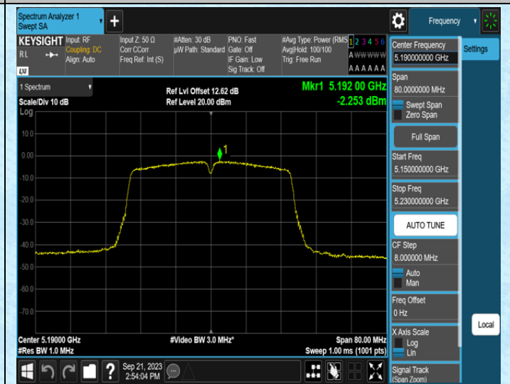
11AC40SISO-Ant1-5190
