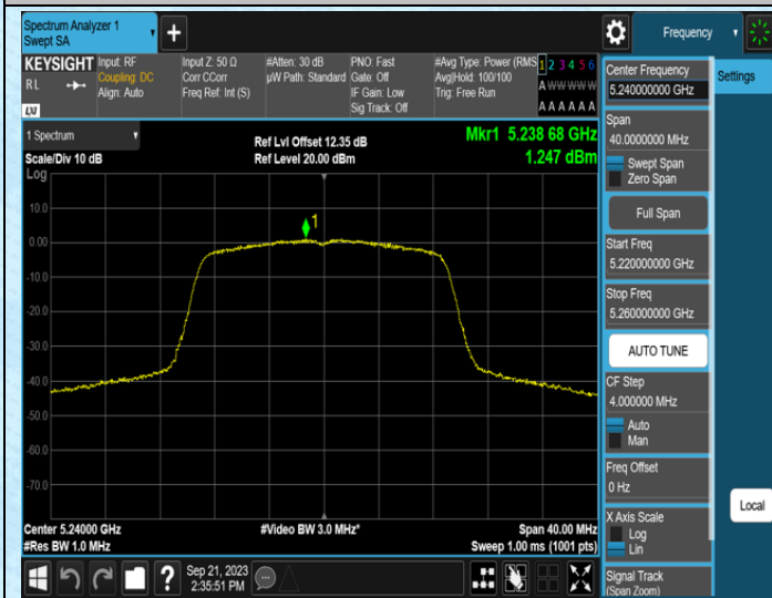
11AC20SISO-Ant1-5240
