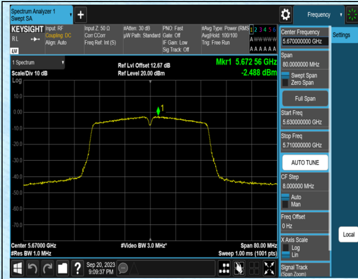
11AC40SISO-Ant0-5670
