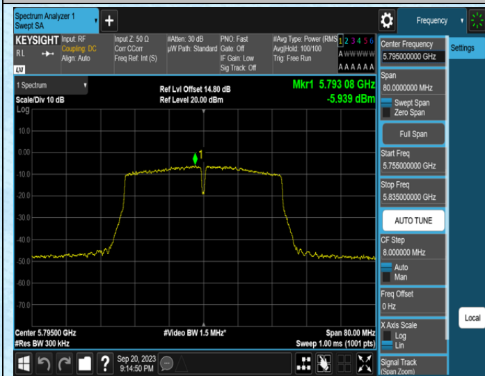
11AC40SISO-Ant0-5795
