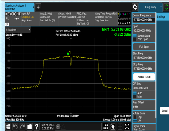
11AC40SISO-Ant1-5755
