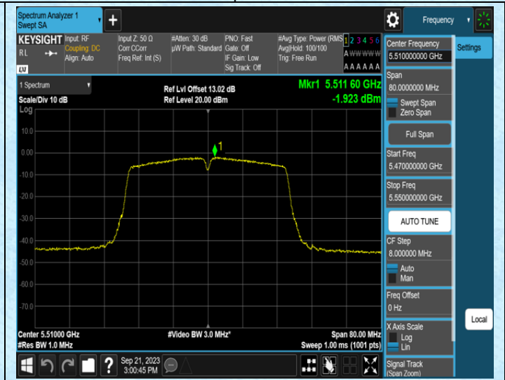
11AC40SISO-Ant1-5510
