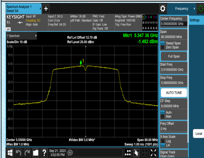
11AC40SISO-Ant1-5550
