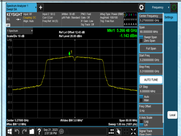
11AC40SISO-Ant1-5270
