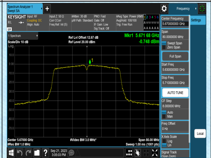
11AC40SISO-Ant1-5670
