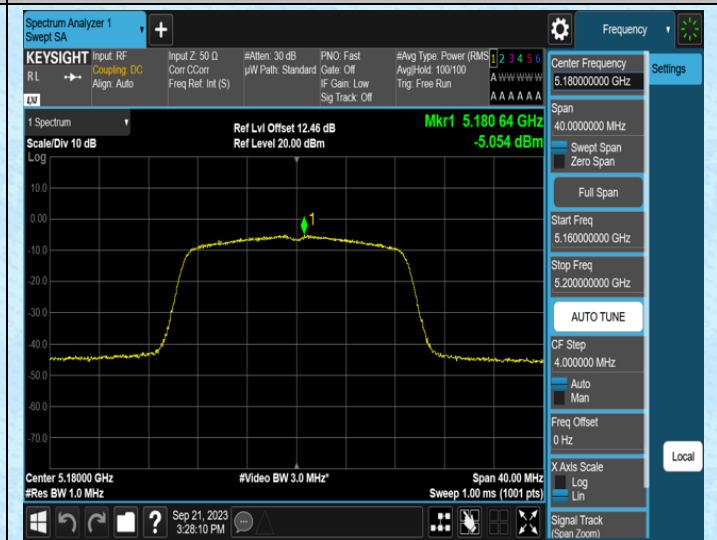
11N20MIMO-Ant1-5180
