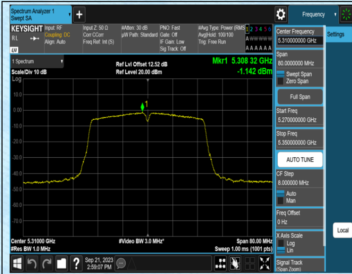
11AC40SISO-Ant1-5310
