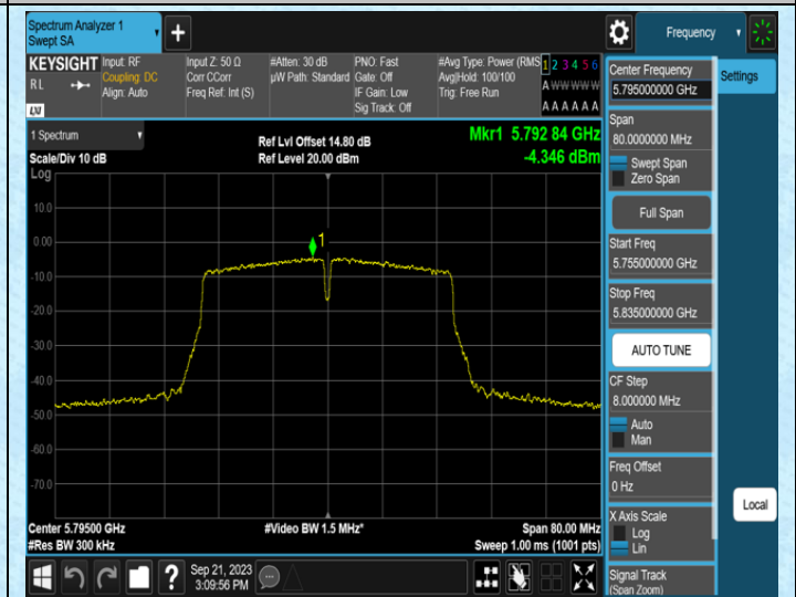
11AC40SISO-Ant1-5795
