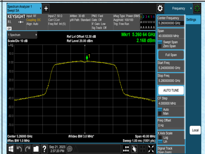
11AC20SISO-Ant1-5260
