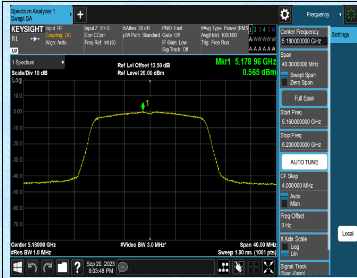
11N20SISO-Ant0-5180
