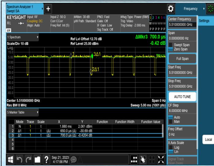
NTNV-11N40MIMO-Ant0-5510
