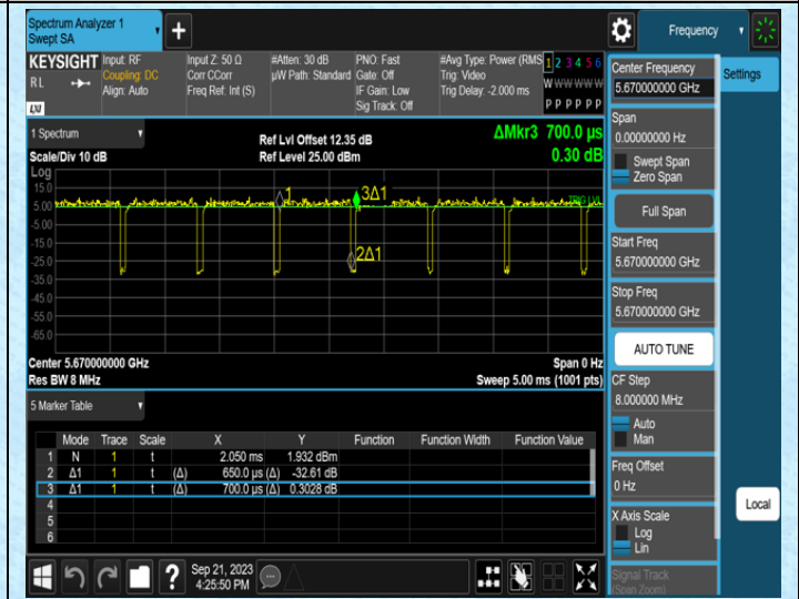
NTNV-11N40MIMO-Ant1-5670
