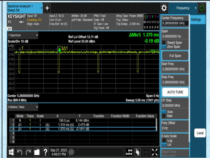
NTNV-11AC20MIMO-Ant1-5260
