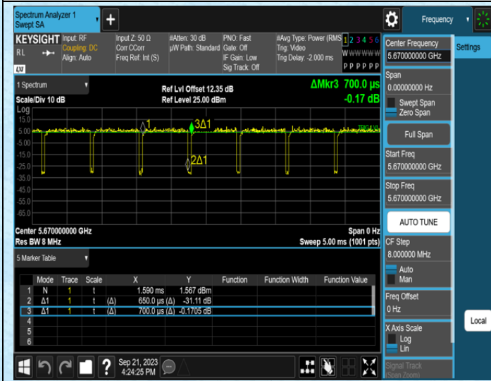
NTNV-11N40MIMO-Ant0-5670
