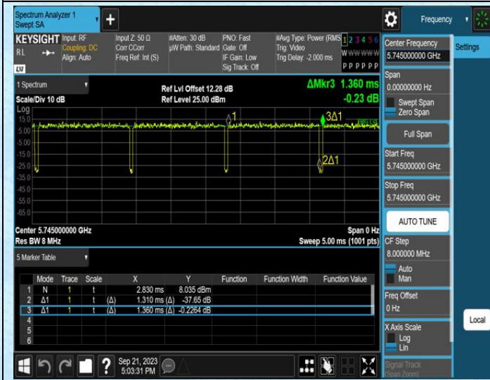
NTNV-11AC20MIMO-Ant0-5745
