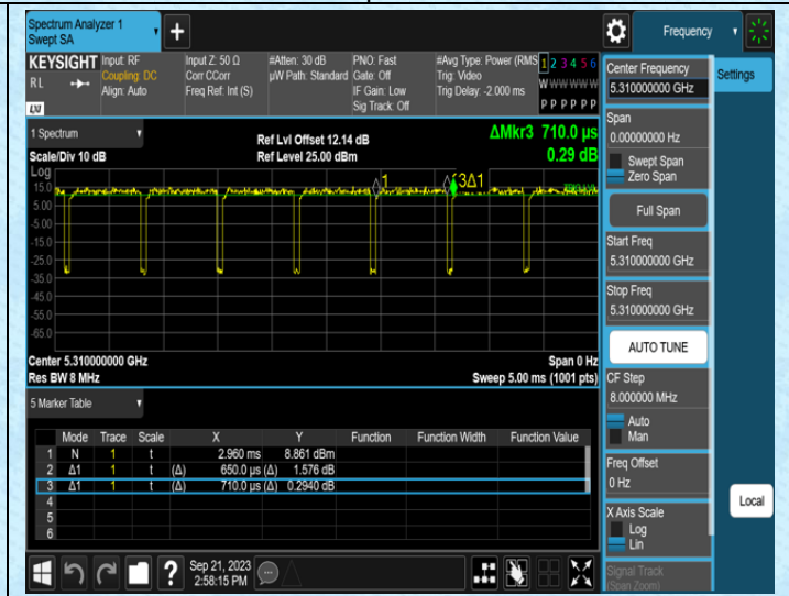
NTNV-11AC40SISO-Ant1-5310
