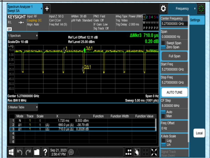
NTNV-11AC40SISO-Ant1-5270
