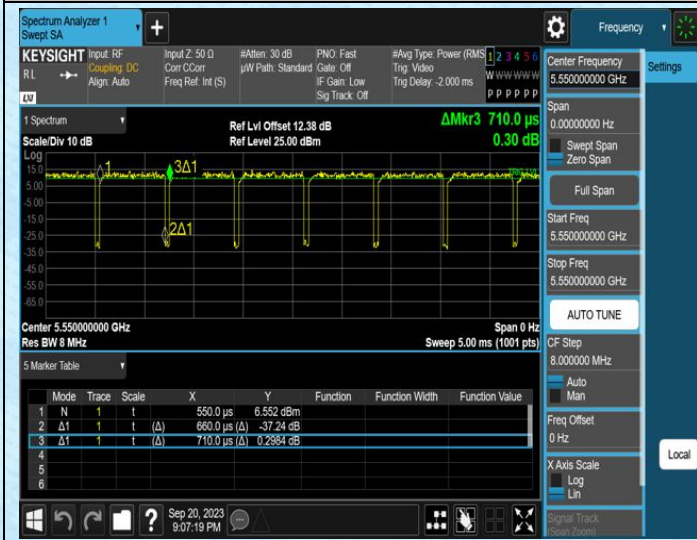
NTNV-11AC40SISO-Ant0-5550
