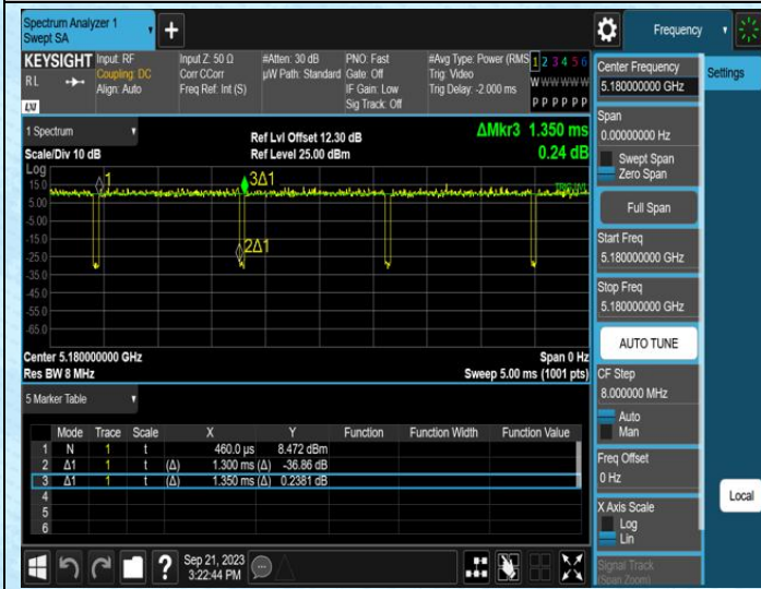
NTNV-11N20MIMO-Ant0-5180
