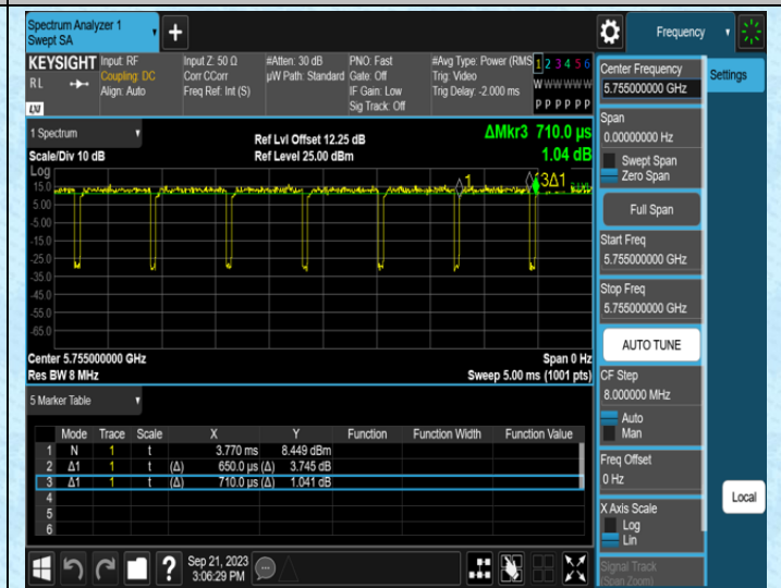
NTNV-11AC40SISO-Ant1-5755
