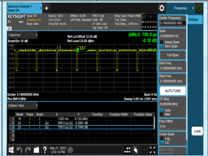
NTNV-11AC40SISO-Ant1-5190
