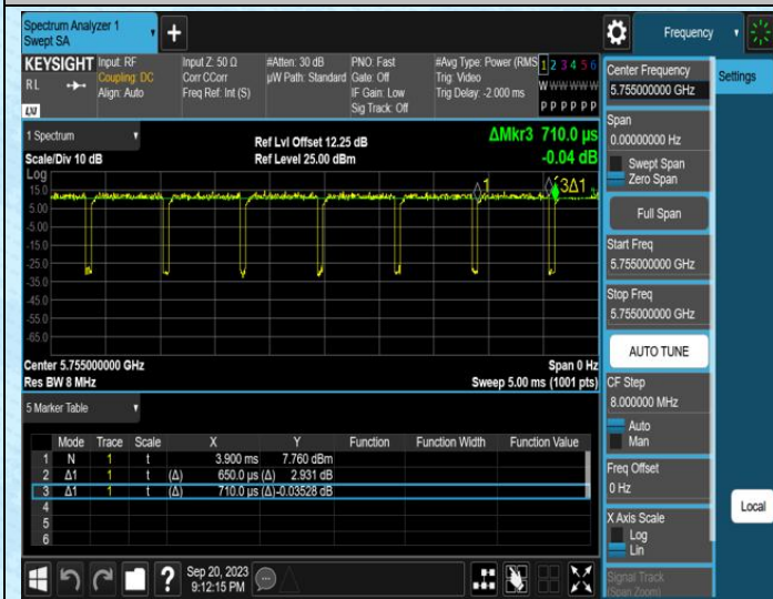
NTNV-11AC40SISO-Ant0-5755
