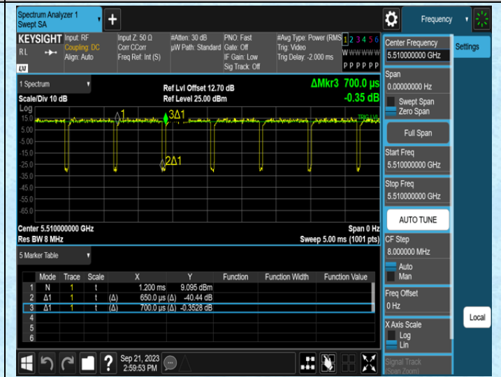
NTNV-11AC40SISO-Ant1-5510
