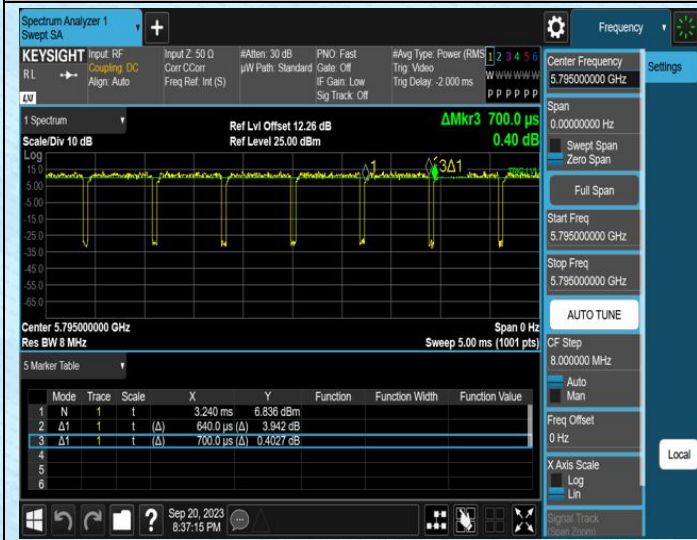
NTNV-11N40SISO-Ant0-5795
