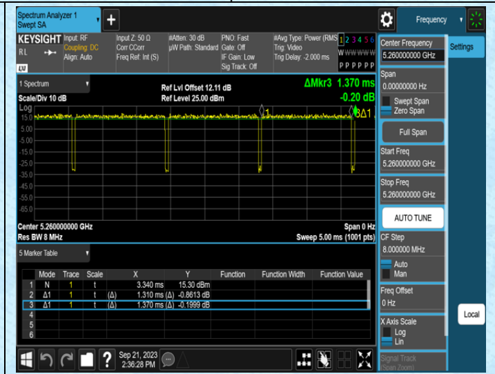
NTNV-11AC20SISO-Ant1-5260
