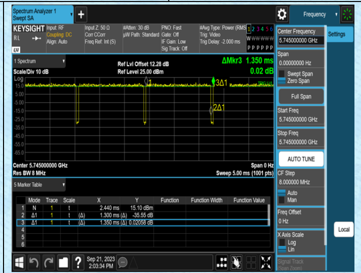
NTVN-11N20SISO-Ant1-5745
