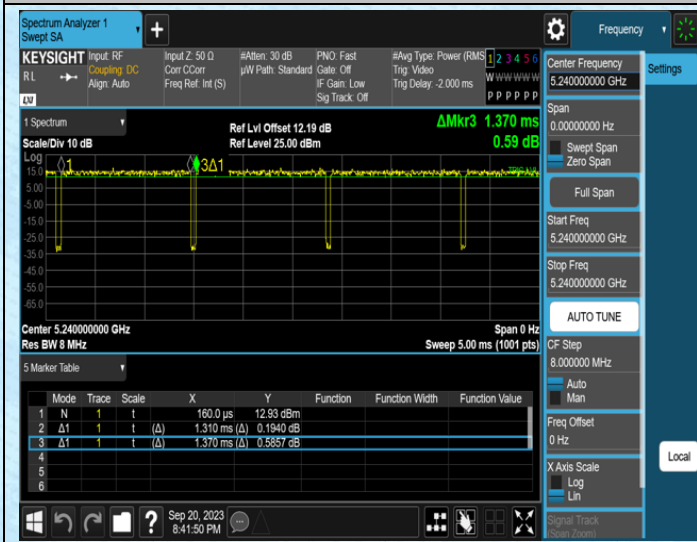
NTNV-11AC20SISO-Ant0-5240
