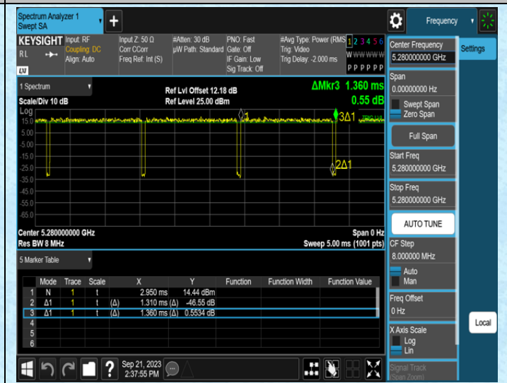
NTNV-11AC20SISO-Ant1-5280
