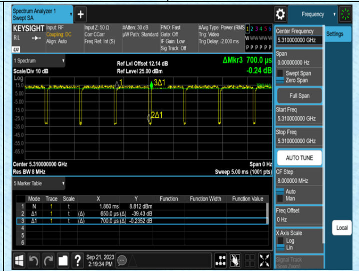
NTVN-11N40SISO-Ant1-5310
