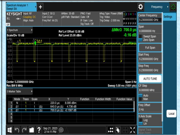
NTVN-11N40SISO-Ant1-5230
