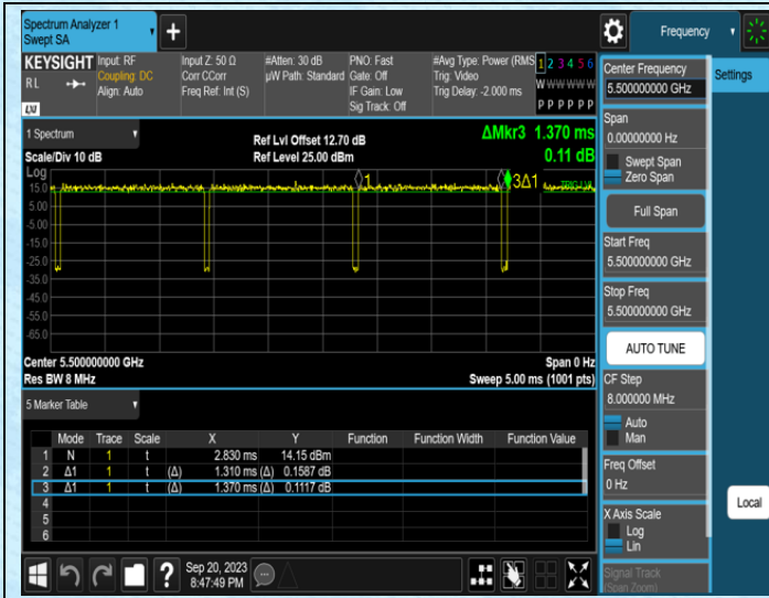
NTNV-11AC20SISO-Ant0-5500
