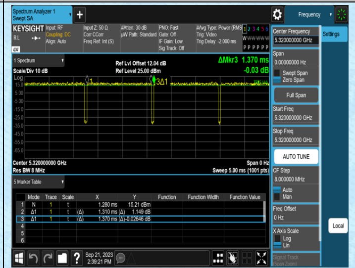
NTNV-11AC20SISO-Ant1-5320
