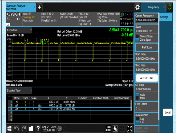
NTVN-11N40SISO-Ant1-5550
