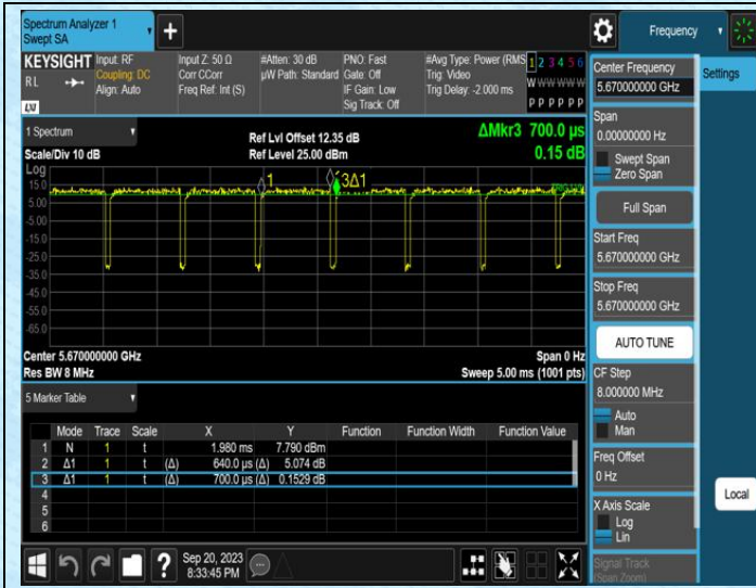
NTNV-11N40SISO-Ant0-5670
