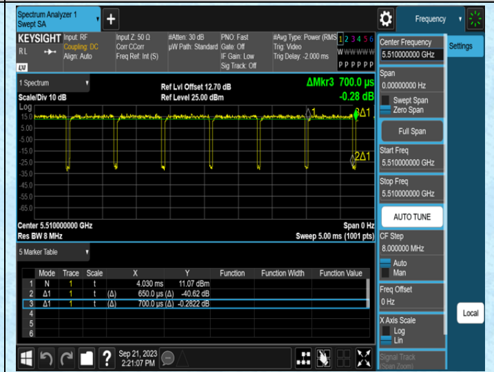
NTVN-11N40SISO-Ant1-5510
