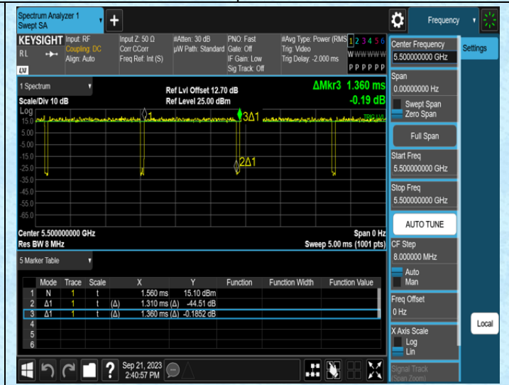
NTNV-11AC20SISO-Ant1-5500
