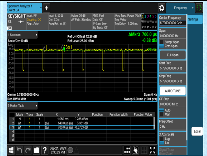
NTNV-11N40SISO-Ant1-5795
