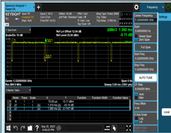
NTNV-11AC20SISO-Ant0-5320
