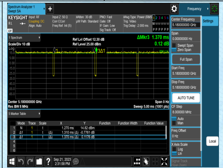
NTNV-11AC20SISO-Ant1-5180
