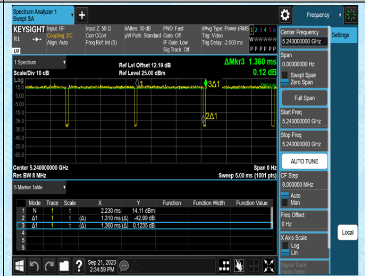
NTNV-11AC20SISO-Ant1-5240
