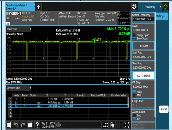
NTNV-11N40SISO-Ant1-5670
