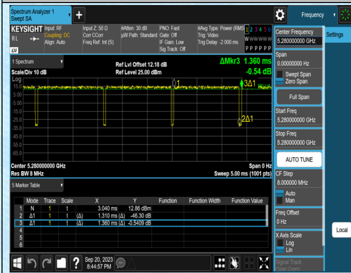
NTNV-11AC20SISO-Ant0-5280
