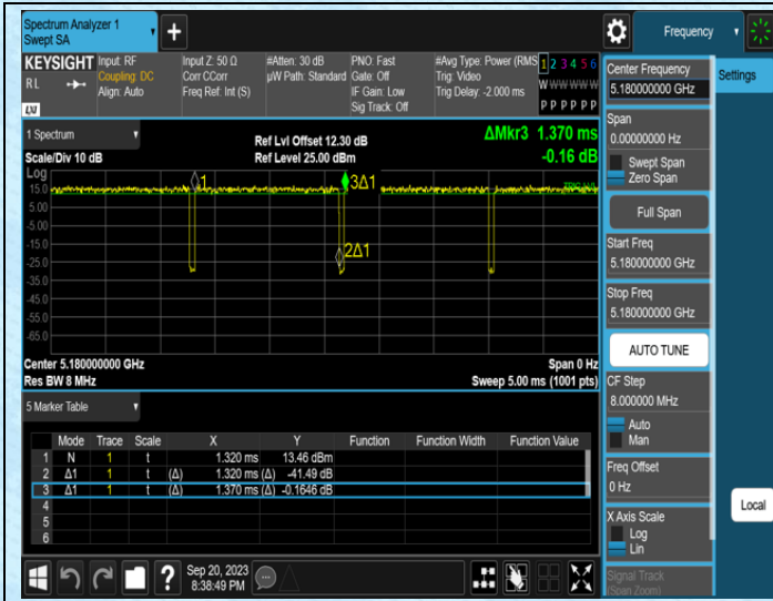
NTNV-11AC20SISO-Ant0-5180
