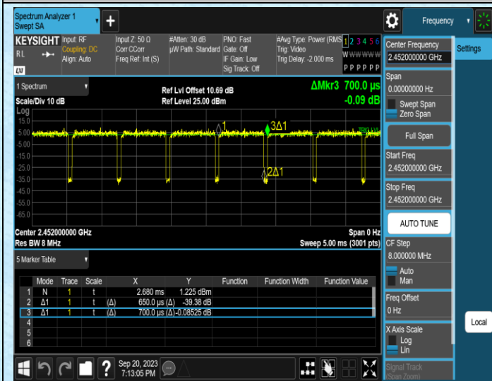
NTNV-11N40MIMO-Ant0-2452
