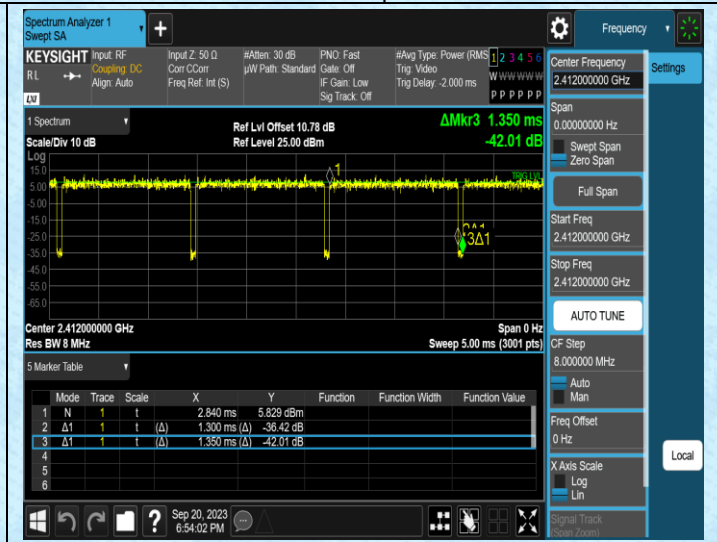
NTNV-11N20MIMO-Ant1-2412
