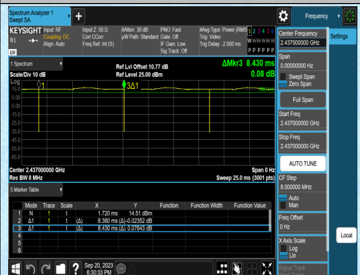
NTNV-11B-Ant1-2437
