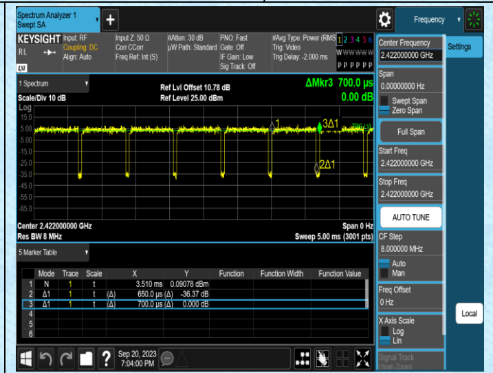
NTNV-11N40MIMO-Ant1-2422
