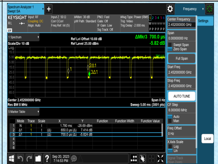
NTNV-11N40MIMO-Ant1-2452
