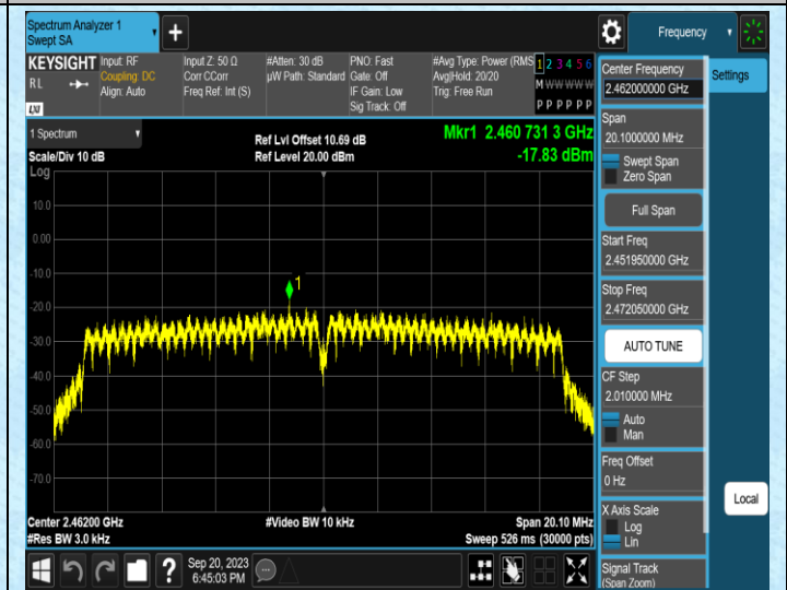
11N20SISO-Ant1-2462
