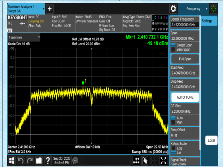
11N20SISO-Ant1-2412
