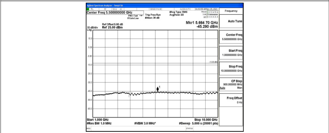
Band12-10MHz-16QAM-23130-1RB#0-Range4:1000~10000MHz
