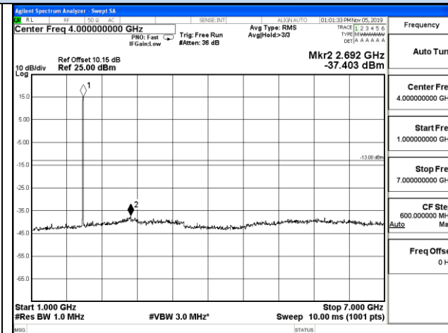
1 GHz – 7 GHz
