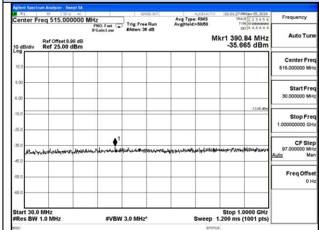
30 MHz – 1000 MHz
