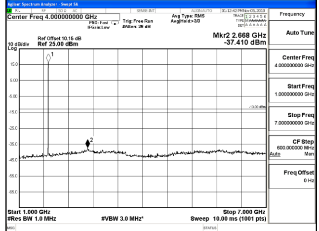
1 GHz – 7 GHz
