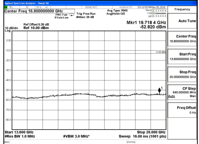
13.6 GHz – 20 GHz
