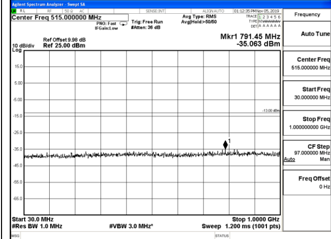
30 MHz – 1000 MHz
