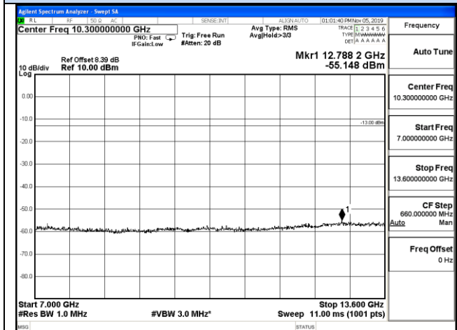
7 GHz – 13.6 GHz
