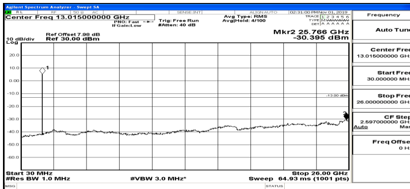
(Channel Bandwidth: 5 MHz)_HCH_16QAM_12RB#0
