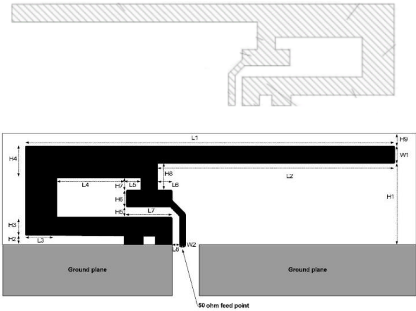
Figure 1. IFA Dimensions
