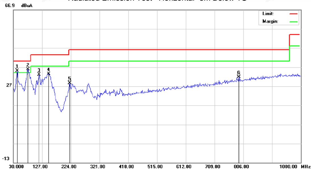
Radiated Emission Test –Horizontal -3m Below 1G
