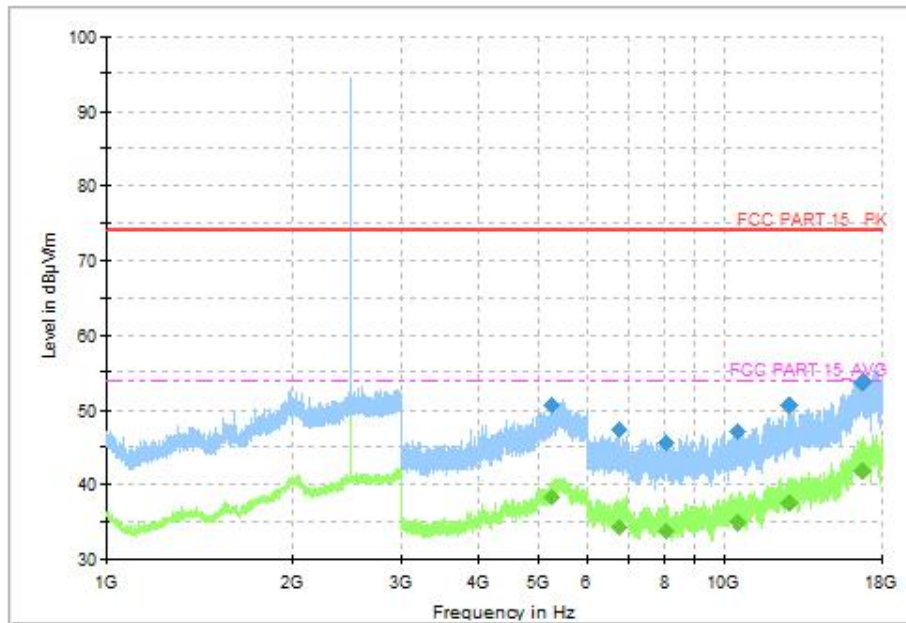
Fig.26 Radiated Spurious Emission (CH39, 1GHz ~18GHz), LE 1M
