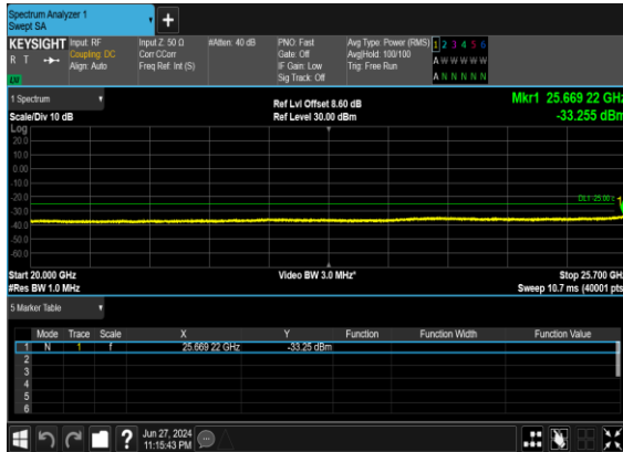
N7(50M)_DFT-s-OFDM_QPSK_Edge_1RB_Left_Mid_CH
