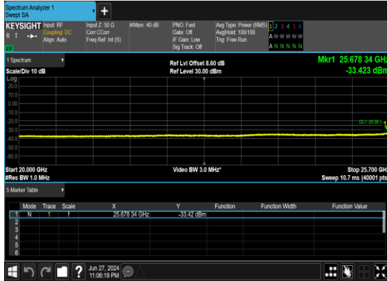
N7(20M)_DFT-s-OFDM_QPSK_Edge_1RB_Left_Mid_CH
