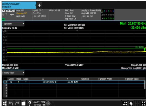
N7(50M)_DFT-s-OFDM_QPSK_Edge_1RB_Left_High_CH
