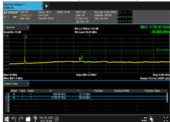
N5(20M)_DFT-s- OFDM_QPSK_Edge_1RB_Left_High_CH
