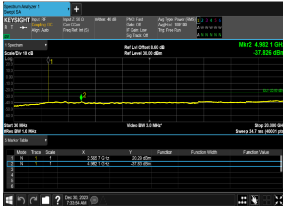
N7(5M)_DFT-s- OFDM_BPSK_Edge_1RB_Left_High_CH
