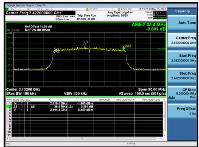
802.11ax-40 MHz(SU) CH3
