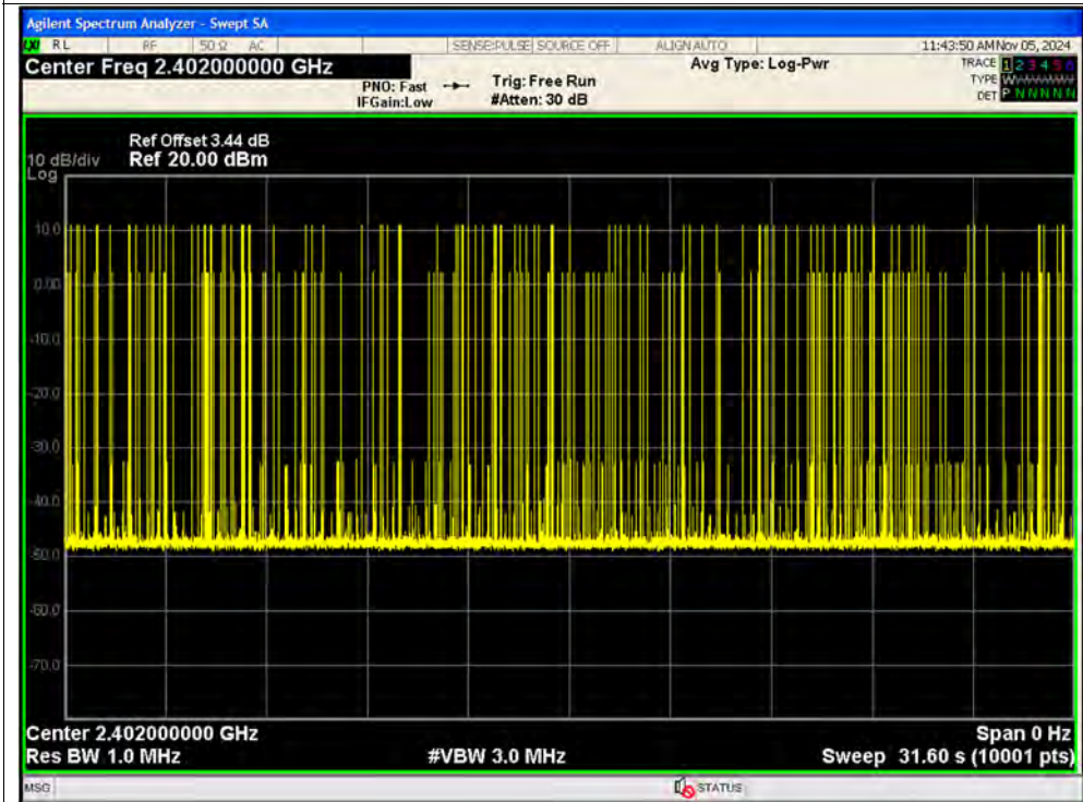
Dwell NVNT 1-DH5 2402MHz Ant1 Accumulated SISO
