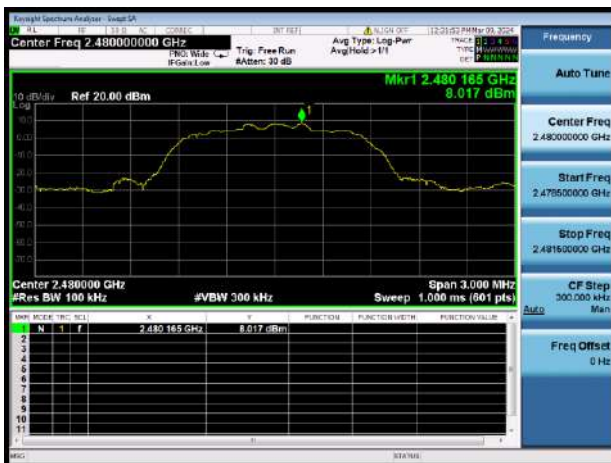
8-DPSK HIGH CHANNEL, CARRIER LEVEL
